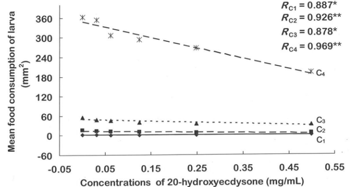
Fig. 2. The correlation between the concentration of 20-hydroxyecdysone in diet and mean food consumption by diamondback moth larvae for each instar. C_1 , C_2 , C_3 , and C_4 represent mean food consumption of 1st, 2nd, 3rd, and 4th instars, respectively. R represents the coefficient; the symbols * and ** next to the coefficient indicate that the correlation between X and Y was significant at P < 0.05 and P < 0.01 , respectively.
