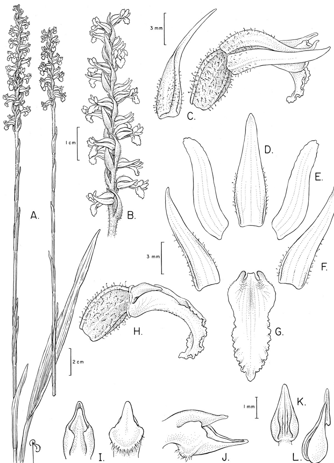
FIG. 2. Spiranthes cernua s. s. A. Habit. B. Inflorescence. C. Flower and floral bract in profile. D–G. Flower, dissected view. D. Dorsal sepal. E. Dorsal petal. F. Lateral sepal. G. Labellum. H. Labellum, column, and ovary in natural position. I–K. Column. I. Dorsal and ventral views. J. Profile. K. Anther. L. Pollinia. Drawn from Pace 612 and Pace 615 by Bobbi Angell.
