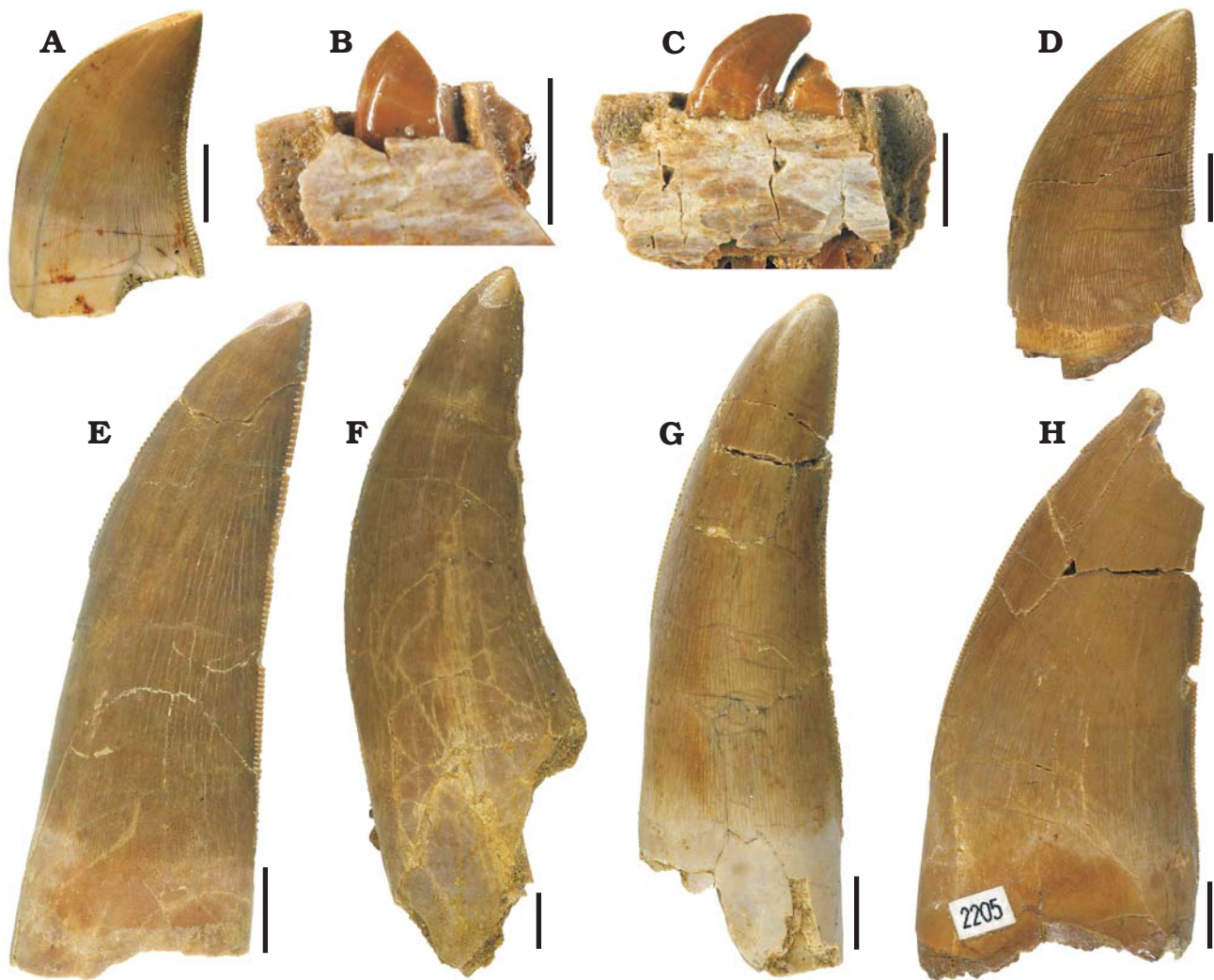
Fig. 2. Theropod dinosaurs teeth from upper Campanian–lower Maastrichtian, Laño. A, D. Theropoda indet. Morphotype 2. A. MCNA 14522. D. MCNA 1853. B, C. ? Pyroraptor olympius Allain and Taquet, 2000. B. MCNA 14623. C. MCNA 14624. E–H. Theropoda indet. Morphotype 1. E. MCNA 1852. F. MCNA 14520. G. MCNA 14521. H. MCNA 2205. All lateral views. Scale bars 5 mm.
