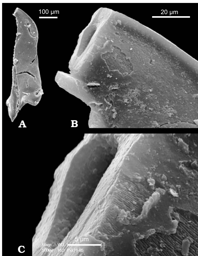
Fig. 3. Internal structure preserved on the weathered surface of the right MI of “ Kettnerites ” sp., ZPAL Sc.8/14.5, sample S.IZ.4 from Ivanje Horizon, Lower Pragian, Podolia.
