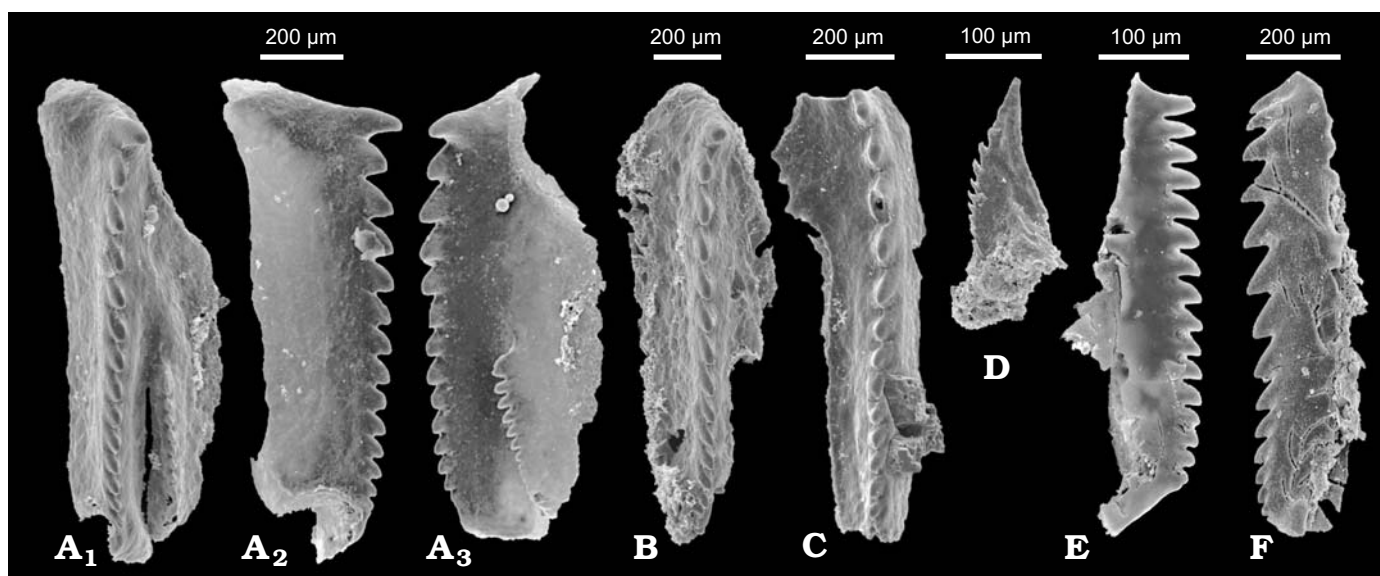
Fig. 4. SEM micrographs of mochtlyellid scolecodonts from Podolia. A–C. Mochtlyella sp. A , lower part of the Borshchiv Horizon, section 48, Lower Lochkovian, sample S.Kh.1. A . ZPAL Sc.8/2.1, right MI in dorsal ( A 1 ), left lateral ( A 2 ), and right lateral ( A 3 ) views. B. ZPAL Sc.8/2.2, incomplete right MI in dorsal view. C. ZPAL Sc.8/2.3, incomplete left MI in dorsal view. D. Mochtlyella ? sp., anterior tooth; lower part of the Borshchiv Horizon, section 48, Lower Lochkovian, sample S.Kh.1, ZPAL Sc.8/2.21. E, F. Mochtlyellidae gen. et sp. indet., undetermined elements MI, upper part of the Ivanye Horizon, section 76, Pragian. E. ZPAL Sc.8/11.5, sample S.IZ.13, incomplete right MI in left lateral view. F. ZPAL Sc.8/8.18, sample S.IZ.13, left MI in right lateral view.
