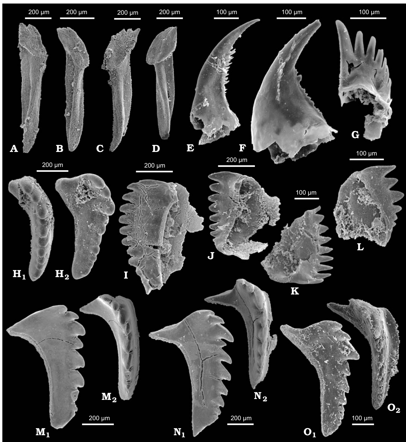
Fig. 7. SEM micrographs of selected elements of paulinitid scolecodonts and undetermined anterior elements from Lower Devonian of Podolia: Ivanye Horizon, section 58 (D, O), section 73 (M, N, K), section 76 (A–C, E, G–J, L); Chortkiv Horizon, section 70 (F). A–D. “ Kettnerites ”? spp. A, B. Left mandibles in dorsal view. A. ZPAL Sc.8/8.19, sample S.IZ.13. B. ZPAL Sc.8/11.14, sample S.Za.2. C, D. Right mandibles in dorsal view. C. ZPAL Sc.8/7.1, sample S.IZ.16. D. ZPAL Sc.8/10.6, sample S.Za.12. E. Family uncertain, gen. et sp. indet. A, ZPAL Sc.8/7.9, sample S.IZ.16, in lateral view. F. Family uncertain, gen. et sp. indet. B, ZPAL Sc.8/4.22, sample S.Zo.4, in lateral view. G. Family uncertain, gen. et sp. indet. C, ZPAL Sc.8/7.18, sample S.IZ.18, in lateral view. H, M–O. “ Kettnerites ”? spp. left MIII. H. ZPAL Sc.8/11.5, sample S.I.Z.18, in dorsal ( H 1 ) and left lateral ( H 2 ) views. M. ZPAL Sc.8/6.6, sample S.Do.6, in right lateral ( M 1 ) and dorsal ( M 2 ) views. N. ZPAL Sc.8/6.7, sample S.Do.6, in left lateral ( N 1 ) and dorsal ( N 2 ) views. O. ZPAL Sc.8/11.13, sample S.Za.12, in left lateral ( O 1 ) and dorsal ( O 2 ) views. I–L. “ Kettnerites ”? spp. left and right MIV. I. ZPAL Sc.8/7.13, sample S.IZ.18, right element in ventral lateral view. J. ZPAL Sc.8/8.22, sample S.I.Z.13, right element in ventral lateral view. K. ZPAL Sc.8/6.15, sample S.Do.2, left element in dorsal lateral view. L. ZPAL Sc. 8/8.8, sample S.IZ.6, left element in ventral lateral view.
