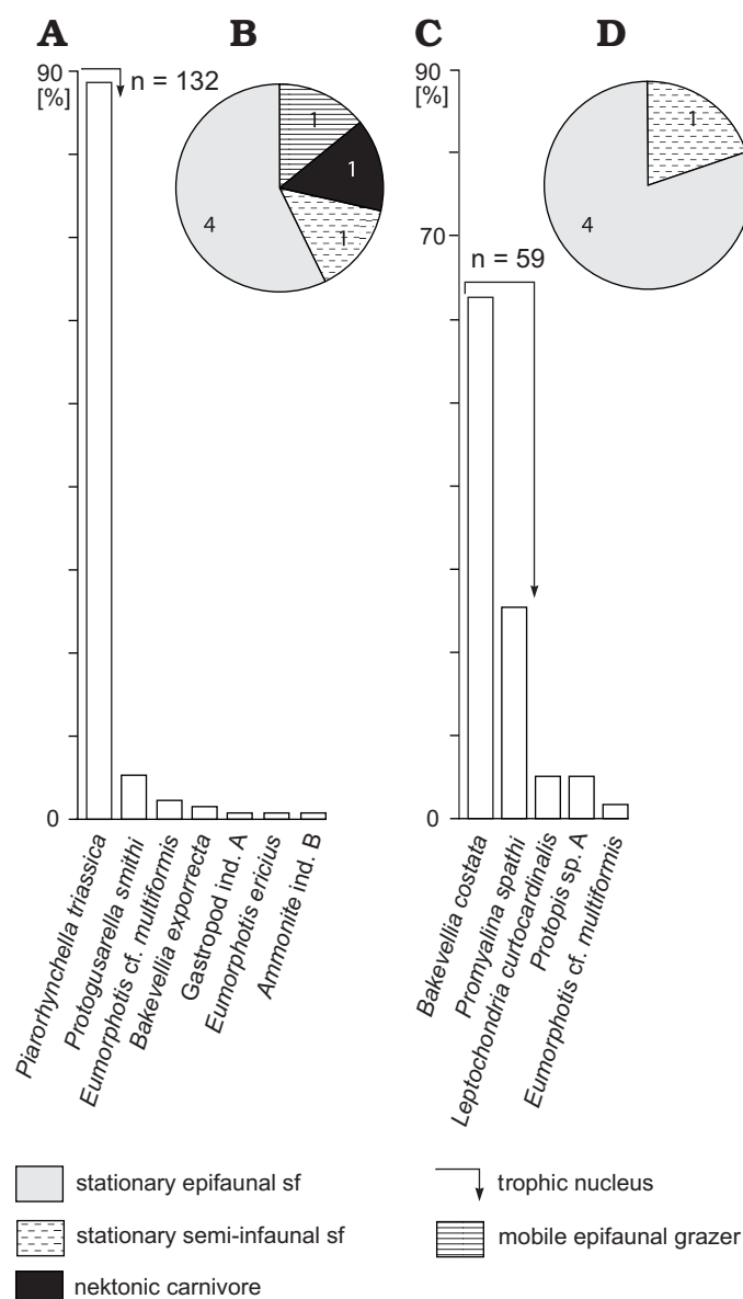
Fig. 15. A, B. Characteristics of the Piarorhynchella triassica Association showing frequency distribution, trophic nucleus ( A ) and ecological structure ( B ). C, D. Characteristics of the Bakevellia costata Assemblage showing frequency distribution and trophic nucleus ( C ) and ecological structure ( D ). The numbers in the pie-chart sections correspond with the species pertaining to each guild.
