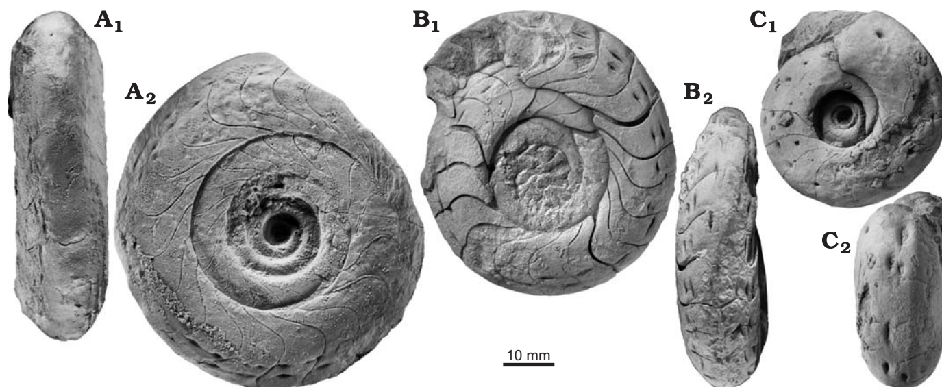
Fig. 3. "Housean pits" type 1. A. Sellanarcestes ebbighauseni Klug, 2002, GPIT 1871-171, Sellanarcestes wenkenbachii Zone, Emsian, northern Jebel Amessoui, Tafilalt, Morocco, from Klug (2002); in ventral ( A_1 ) and lateral ( A_2 ) views. B. Sellanarcestes cf. ebbighauseni Klug, 2002, PIMUZ 28582, Sellanarcestes wenkenbachii Zone, Emsian, Jebel Ouafouilal, Tafilalt, Morocco; in lateral ( B_1 ) and ventral ( B_2 ) views. C. Large pits in Anarcestes sp., PIMUZ 28581, late Emsian, Jebel Mech Agrou, Tafilalt, Morocco; in lateral ( C_1 ) and ventral ( C_2 ) views. All specimens coated with NH_4Cl .
