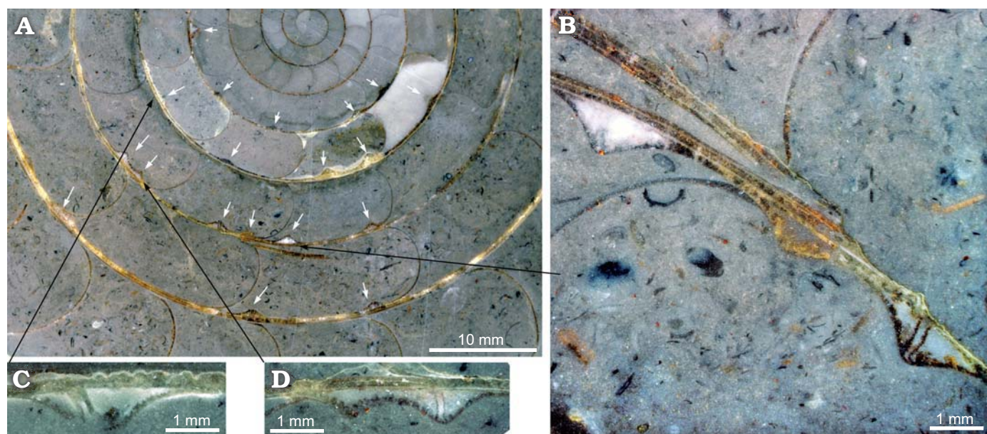
Fig. 7. Longitudinal section through the well preserved specimen PIMUZ 28583 of Sellanarcestes spp., Sellanarcestes wenkenbachi Zone, Emsian, Oufrane (S of Tata), Morocco. A. +/- median section displaying many "Housean pits", most with internal tube; overview. "Housean pits" are marked by white arrows. B. Three closely spaced pits, two displaying the internal tubes, the remaining void inside the pit is filled with a fine-grained sparitic matrix, note the continuous ammonoid shell layer covering the pits and the septum, which grew on the pit wall, note the distinguishable shell layers, which are recrystallised to varying degrees. C. A corroded pit with tube, note the continuation of the innermost ammonoid shell layer. D. Two adjacent fused pits, only the right pit shows the delicate internal tube, mural part of septum on the left.
