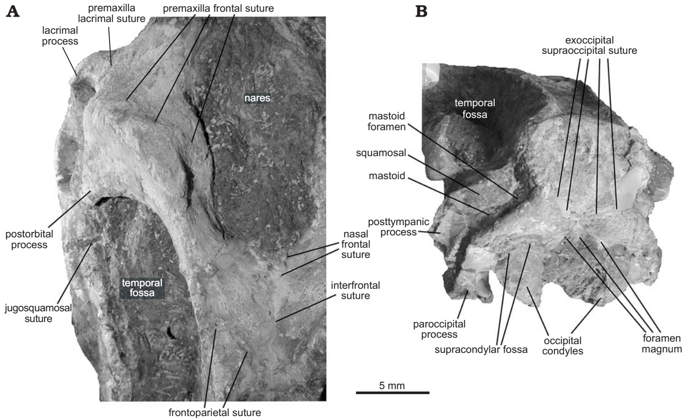
Fig. 2. Nasal opening and superior left orbit (A) and oblique occipital view (B) of the sirenian Domningia sodhae gen. et sp. nov. (IITR-SB 3091), Khari Nadi Formation, Aquitanian (lower Miocene), Nangia, District Kutch, India.
