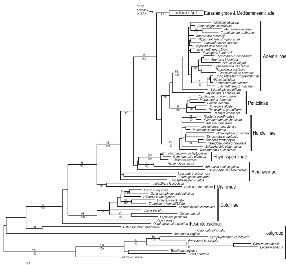
Fig. 1. Basal part of a phylogenetic tree from a maximum-likelihood (ML) analysis of nrDNA ITS sequence variation data based on the TrN + \Gamma model of DNA substitution (Tamura & Nei 1993) with base frequencies, gamma distribution parameter \alpha and substitution rate matrix given in the text. Values above branches indicate bootstrap support values from a maximum-parsimony (MP) analysis based on 100 replicates and values below branches give posterior probability (PP in percent) of clades gained from a Bayesian analysis (BI) of data.
