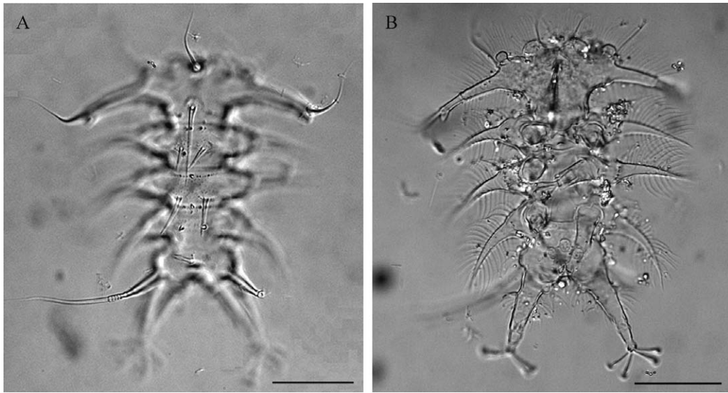
Fig. 3. Neostygartus lovedeluxe n. sp. DIC micrograph of the holotype. (A) Dorsal view. (B) Ventral view. Scale bar = 50 \mu\text{m} .
