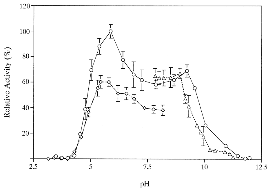
Fig. 7. Effect of pH on the purified endo-β-1,4-glucanase activity. Activity was measured using (○) acids mixture - NaOH, (◇) phosphate - citrate, or (△) boric acid, KCl - sodium carbonate buffer.
