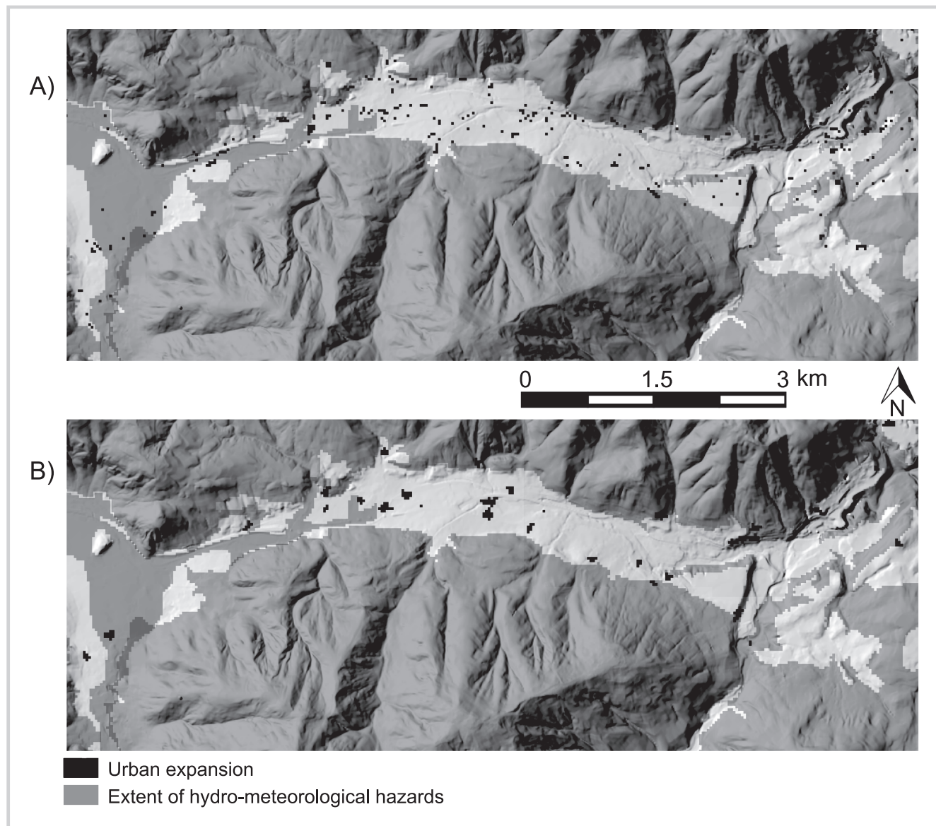
FIGURE 5 Projected impact of expansion on exposure to hydro-meteorological hazards in the tourism area near Tarvisio. (A) Business-as-usual scenario; (B) alternative scenario.
