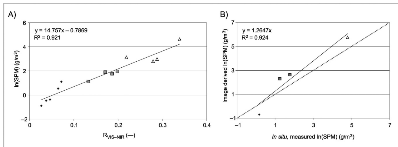
FIGURE 3 (A) Natural logarithmic of SPM concentrations versus AVNIR-2 atmospherically corrected reflectance data ( R_{VIS-NIR} ). The regression line was used to map SPM concentrations from satellite data in the whole image; (B) comparison of satellite-derived and in situ measured SPM concentrations for the 4 lakes in China. In both plots symbols change according to water colors (hence to water reflectance and SPM concentrations): diamonds for dark blue lakes; squares for turquoise lakes; triangles for light gray lakes.
