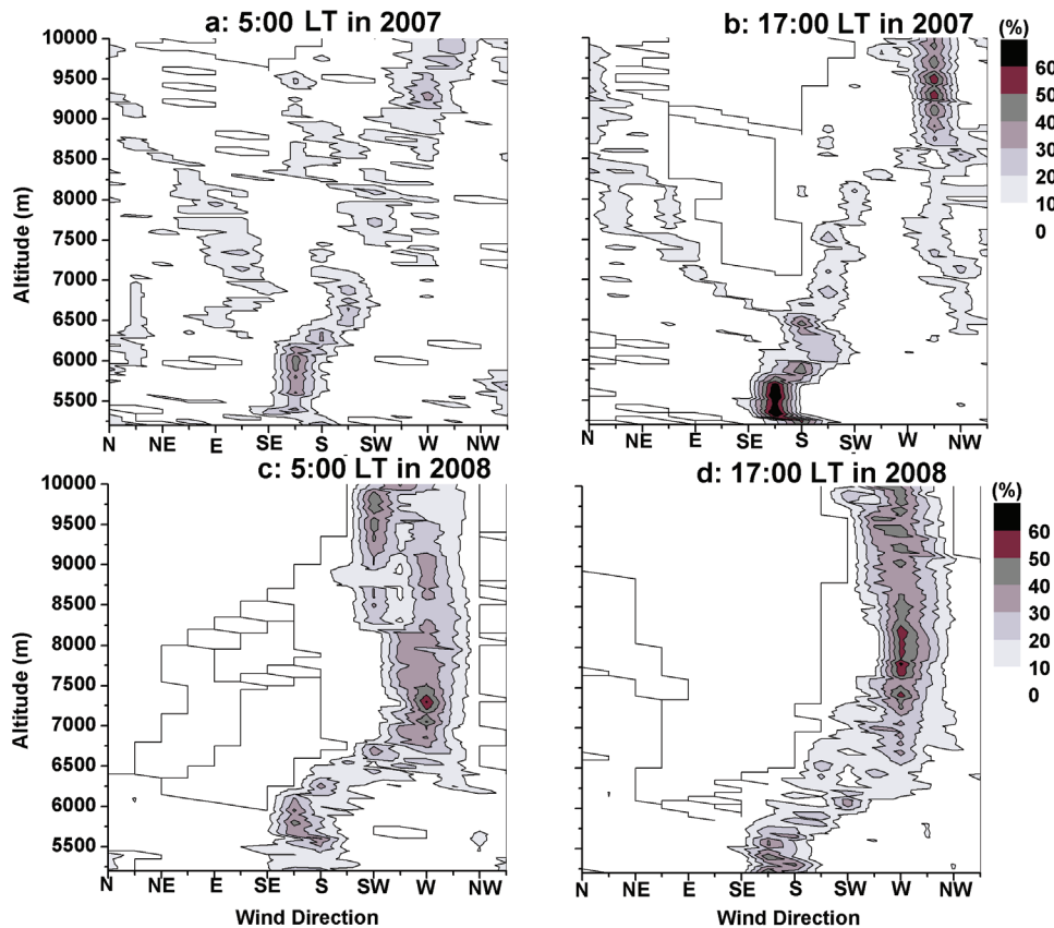
FIGURE 5. Mean variations of wind directions between altitudes of 5200 and 10,000 m a.s.l. at 5:00 and 17:00 local time (LT) over the periods from middle April to early May of 2007 and 2008.
