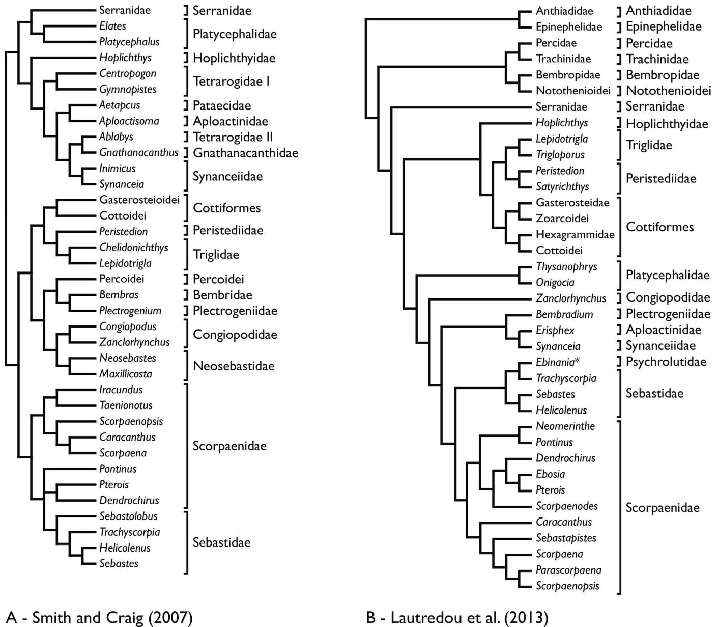
Fig. 2. Molecular hypotheses of inter- and intrafamilial relationships of the scorpaenoid lineage and allies: (A) Scorpaenoidei and allies (Smith and Craig, 2007); (B) traditional Scorpaeniformes and allies (Lautredou et al., 2013; * indicates probable problematic placement—see Smith and Busby [2014] for discussion).
