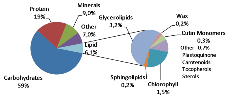
Figure 21. Relative Distribution of Lipids and Other Components of Arabidopsis Leaf.
