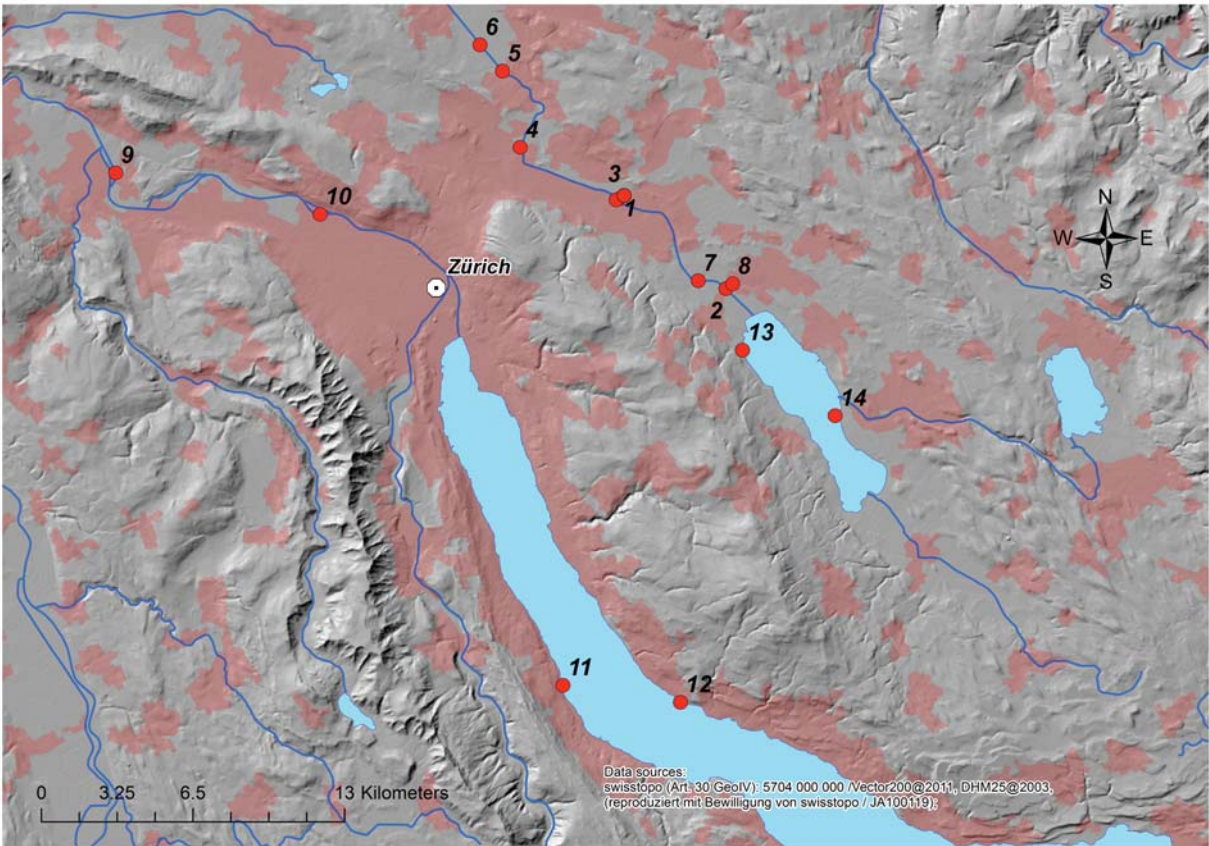
Figure 1. Locations of sampling sites in the northeastern part of Switzerland. All sites were in the drainage systems of the river Glatt and river Limmat and Lake Zurich and Greifensee and Lake Zurich, respectively. Blue areas represent main water bodies and rivers, whereas red areas represent settlements in the relief map (gray). Numbers correspond to sites listed in Table S1.
