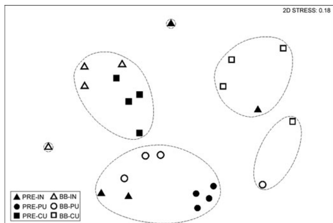
FIGURE 6. Multidimensional scaling (MDS) plot of the macroinfaunal assemblages for each combination of estuary (Biloxi Bay estuary [BB]; Pascagoula River estuary [PRE]) and landscape type (IN = intact natural; PU = partially urbanized; CU = completely urbanized). The dashed contour identifies significant groupings (40% similarity) based on agglomerative hierarchical clustering and similarity profiles.
