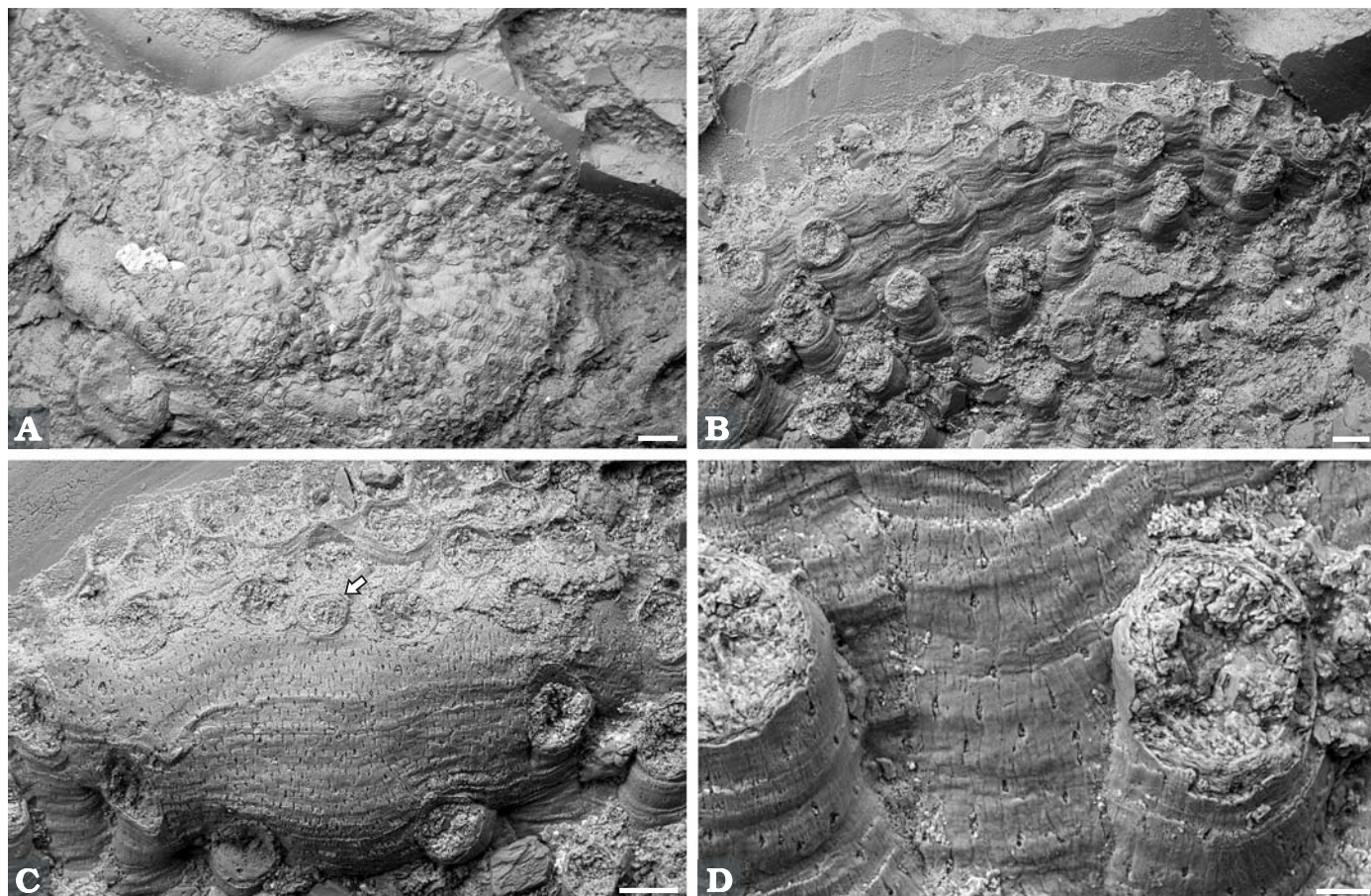
Fig. 12. Plagioeciid cyclostome bryozoan Hyporosopora tenera (Reuss, 1867) from the Middle Jurassic ore-bearing clays of the Polish Jura, GIUS 8-3509-12. A. Colony view. B. Marginal autozooids. C. Gonozooid with ooeciopore (arrowed). D. Pseudopores. Scale bars: 300 µm (A), 100 µm (B, C), 30 µm (D). BSE SEM images of uncoated specimens.
