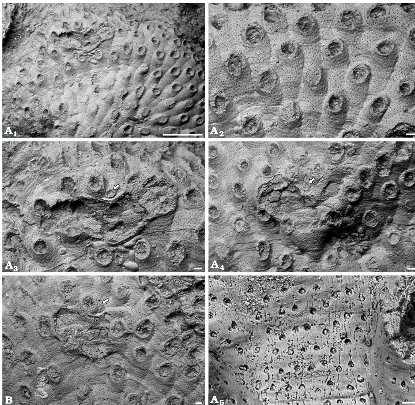
Fig. 13. Plagioeciid cyclostome bryozoan Hyporosopora aff. sauvagei (Gregory, 1896) from the Middle Jurassic ore-bearing clays of the Polish Jura. A. Middle Bathonian, Bugaj, GIUS 8-3509-22. A 1 , colony view; A 2 , autozooids; A 3 , boomerang-like gonozooid, ooeciopore arrowed; A 4 , heart-shaped gonozooid, ooeciopore arrowed; A 5 , pseudopores. B. Middle Bathonian, Bugaj, NHM BZ 5612(2), subtriangular gonozooid, ooeciopore arrowed. Scale bars: 1 mm (A 1 ), 100 µm (A 2 –A 4 , B), 20 µm (A 5 ). BSE SEM images of uncoated specimens.
