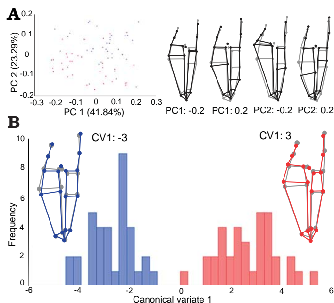
Fig. 8. Cross-plot of the first two principal components (labeled with their corresponding eigenvalues) and wireframes (A) and canonical variation plot (using chirality membership as the group defining criterion) and wireframes (B) for Idiognathodus luganicus . Black wireframes, form with values of the corresponding principal component values; gray wireframes, mean form provided by the preliminary Procrustes fit; blue/red wireframes, form achieved with values of the corresponding canonical variate; blue, sinistral; red, dextral.
