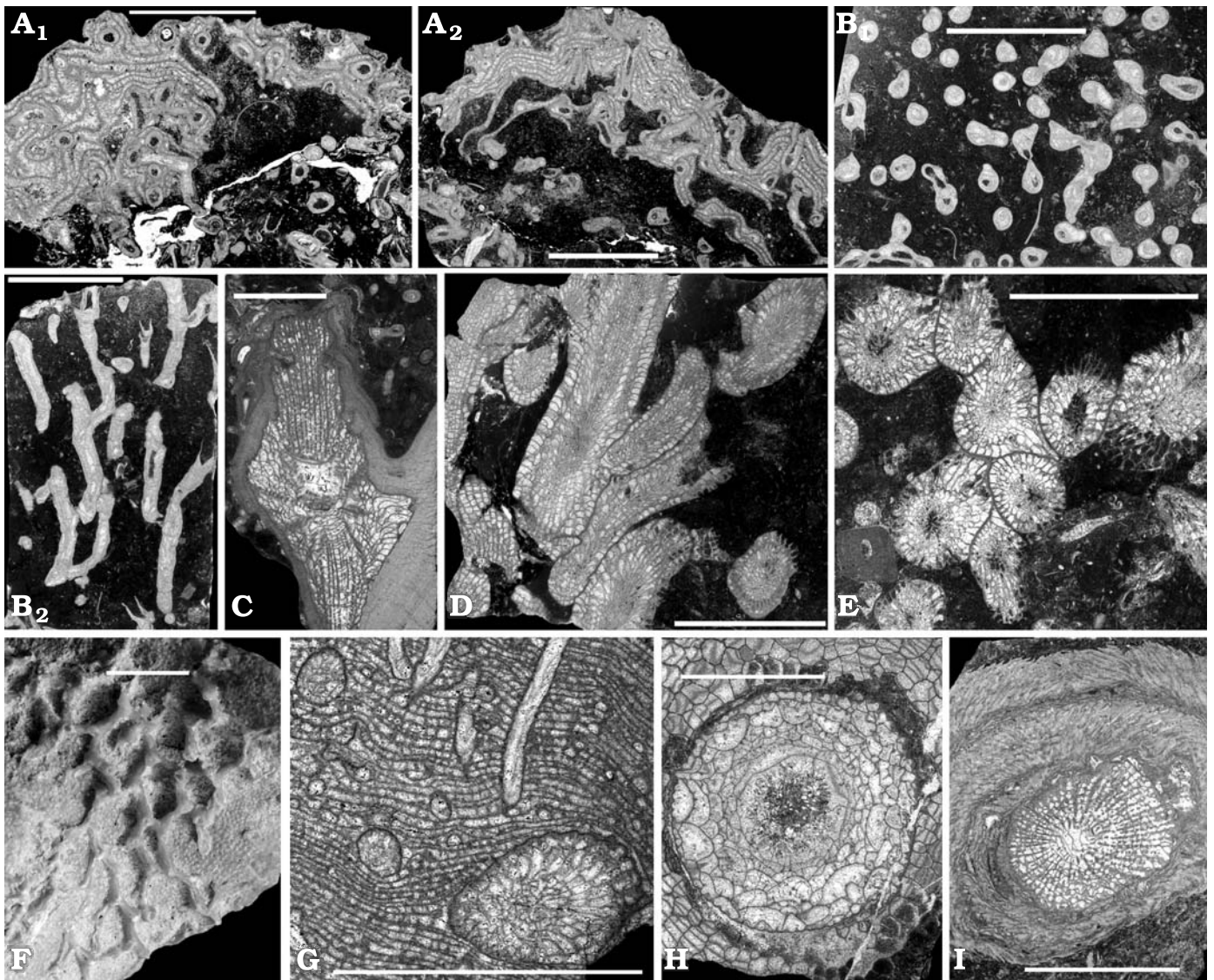
Fig. 10. Thin section photographs of tabulate and rugose corals from Katri biostrome, upper Ludlow, Silurian, showing the identifications of taxa. A. Syringopora multifaria Klaamann, 1962 in symbiosis with stromatoporoid Petridiostroma convictum Yavorsky, 1929, GIT656-51, transverse ( A 1 ) and vertical ( A 2 ) sections. B. Syringopora multifaria , GIT656-105, transverse ( B 1 ) and vertical ( B 2 ) sections. C. Vertical section of Hedstroemophyllum growing on stromatoporoid, GIT656-16. D. Different sections through corallites of Stereoxylodes , GIT656-50. E. Different sections through corallites of Entelophyllum , GIT656-41. F. Aulopora amica Klaamann, 1962 encrusting another coral, GIT656-62. G. Transverse section of Stauria in symbiosis with stromatoporoid Petridiostroma convictum , GIT656-47. H. Transverse section of Cystiphyllum in tabulate Favosites forbesi Milne-Edwards and Haime, 1851, GIT656-72. I. Transverse section of Hedstroemophyllum encrusted by Kitakamiia callosa Klaamann, 1964, GIT656-60. Scale bars 10 mm.
