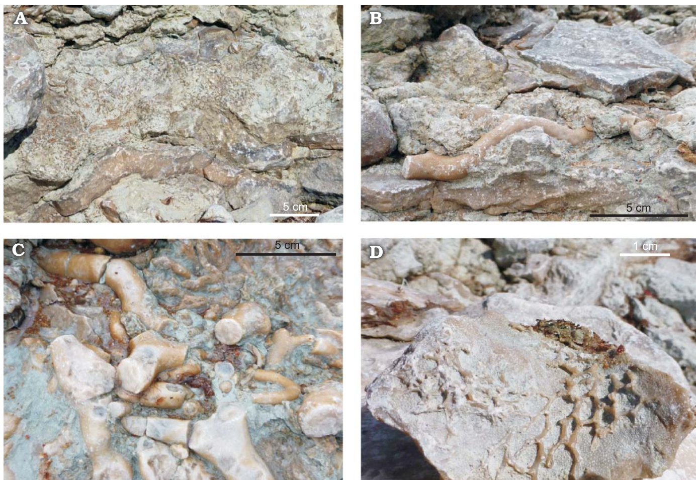
Fig. 5. Field photographs of Facies 2 in Katri biostrome, upper Ludlow, Silurian. A. Laminar Syringostromella borealis Nicholson, 1891 in lower centre of photo, surrounded by grey-green wackestone. B. Broken stem of Laceripora in centre, with laminar stromatoporoids above and below it. C. Fragmented Laceripora , and the edges of two small bulbous stromatoporoids at the top of the photo. D. Encrusting aulopodid tabulate on the upper surface of a laminar tabulate coral.
