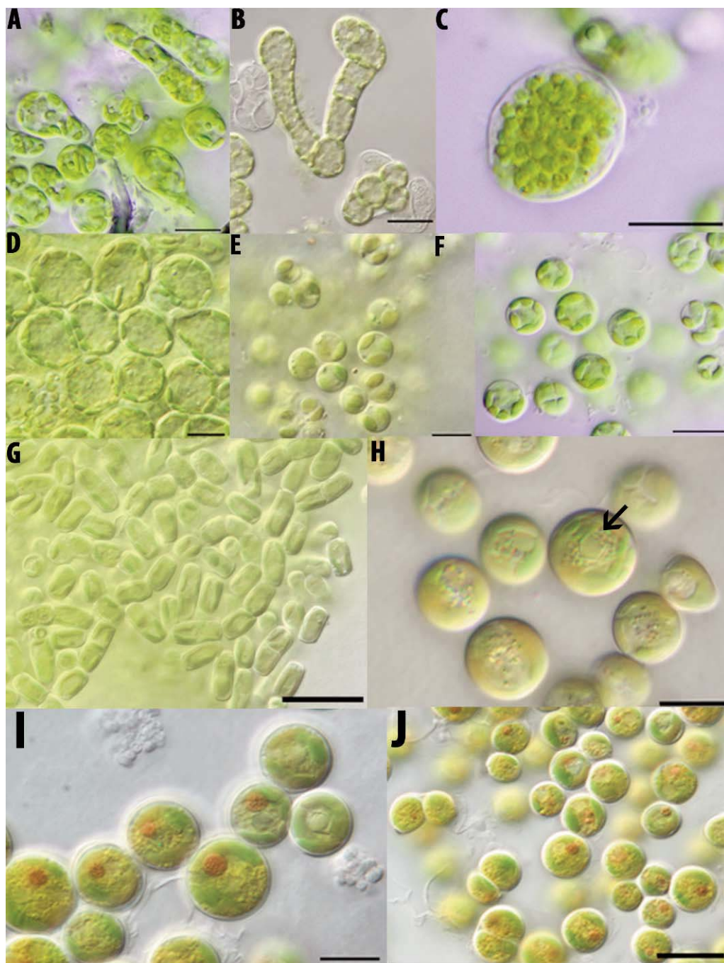
Fig. 8. Representative xanthophyte and eustigmatophyte taxa (strain numbers are indicated in parentheses). Panels A–D, Capitularia : A , short filaments with bulbous end (WJT43VFNP18B); B , short filament and individual cells (WJT43VFNP32); C , sporangium with zoospores (WJT43VFNP32); D , vegetative cells with multiple pyrenoids and free zoospores at lower left (WJT43VFNP32). Panels E–F Pleurococcus : E , vegetative cells with lobed chloroplast and sporangia producing 4 daughter cells (WJT43VFNP24); F , vegetative cells and sporangia (WJT40VFNP19). Panel G , Xanthonema (WJT36VFNP5). Panels H–J, Eustigmatos : H , vegetative cells with pyrenoid indicated by arrow (WJT66VFNP74); I , vegetative cells showing pigment and lobed chloroplast (WJT24VFNP32); J , vegetative cells and dividing cells (WJT24VFNP32). Panels A–D, F–G, and I–J: scale bar = 10 \mu\text{m} ; panels E and H: scale bar = 5 \mu\text{m} .
