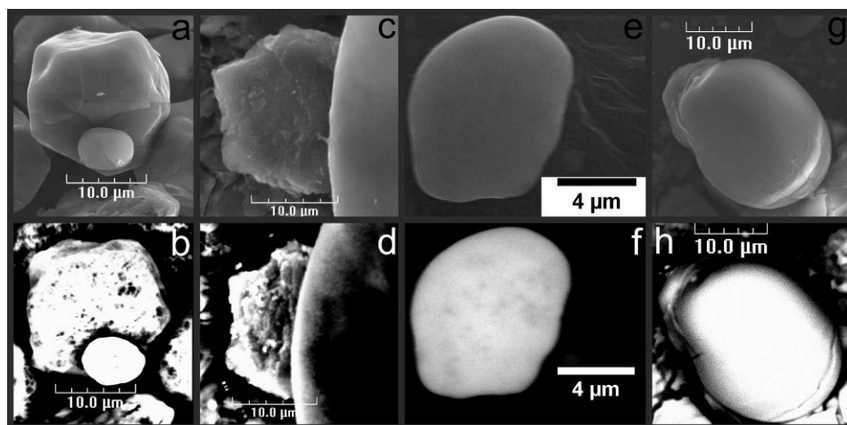
Figure 4. SEM micrographs of starch from: (a) Zea mays kernel under SE (secondary electrons), (b) Zea mays kernel under BSE (backscatter electrons), (c) Zea mays pollen under SE, (d) Zea mays pollen under BSE, (e) Nothoscordum bivalve bulb under SE, (f) Nothoscordum bivalve bulb under BSE, (g) Nothoscordum bivalve pollen under SE, and (h) Nothoscordum bivalve pollen under BSE. Note that the starch granule in micrographs a and b is overlain by a smaller starch granule and the Zea mays starch granule in c and d is partly covered by a pollen grain. The white edge of the pollen grain under BSE in d is due to the edge-effect (Kotera et al. 1990).
