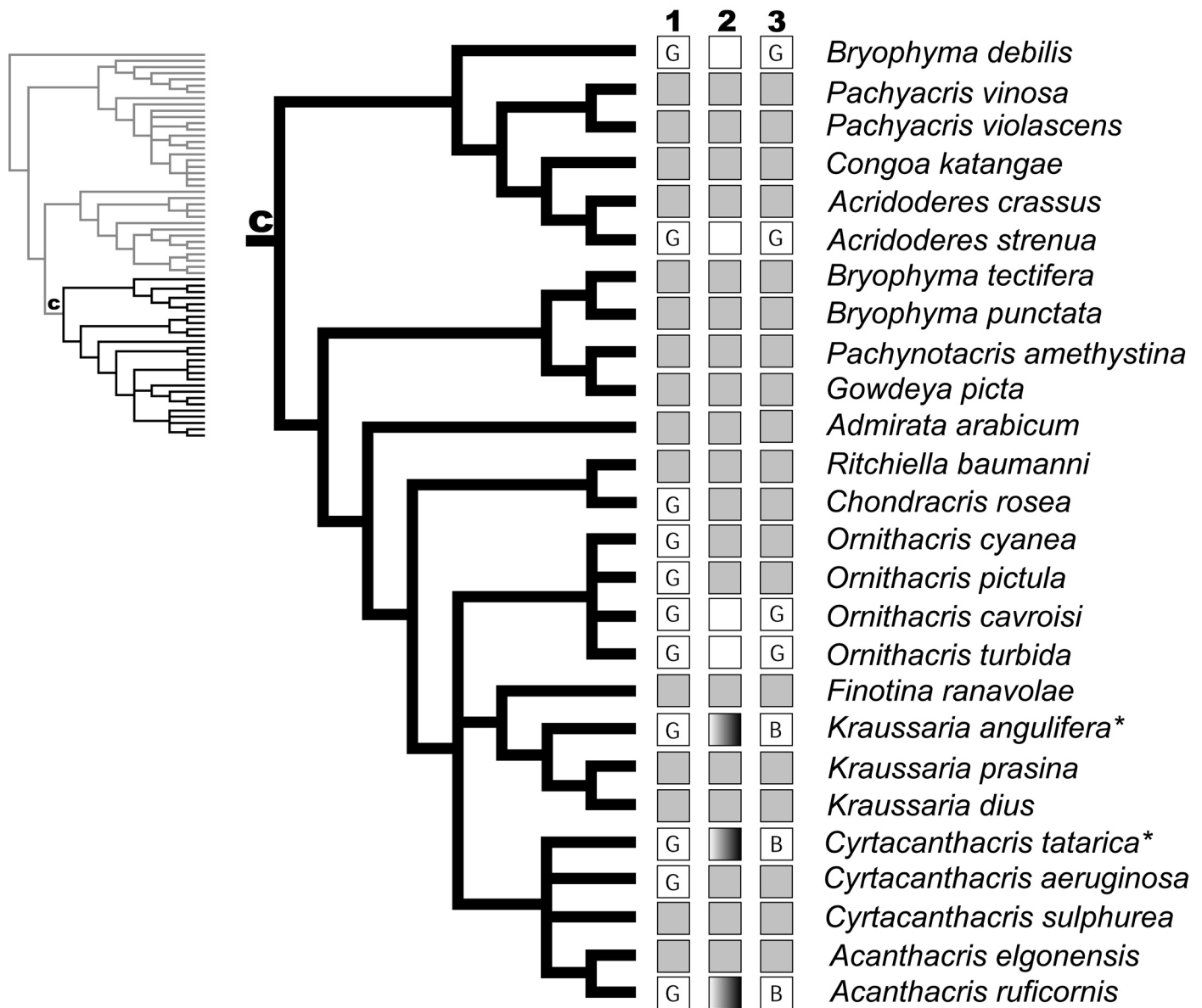
Fig. 4. Character mapping analysis of chromatic plasticity for clade C. See Fig. 2 legend for the explanation of the color coding. Bryophyma is not monophyletic. Four species shown here do not change color when crowded, which is unique for the subfamily. Subspecies of Cyrtacanthacris tatarica and C. aeruginosa were collapsed to single terminals.
