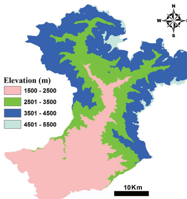
FIGURE 3. Elevation zones of the Lidder watershed.
