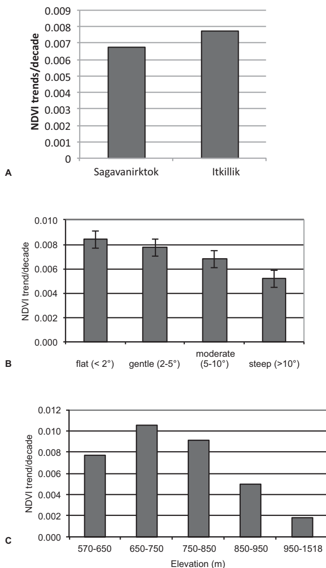
FIGURE 6. NDVI trend (units \times decade ^{-1} ) for areas of (A) two major glacial ages, mid-Pleistocene Sagavanirktok glaciation and late Pleistocene Itkillik glaciation; (B) different steepness; and (C) different elevations in an area of the foothills of the Brooks Range, Alaska, based on Landsat data from 1985 to 2007.
