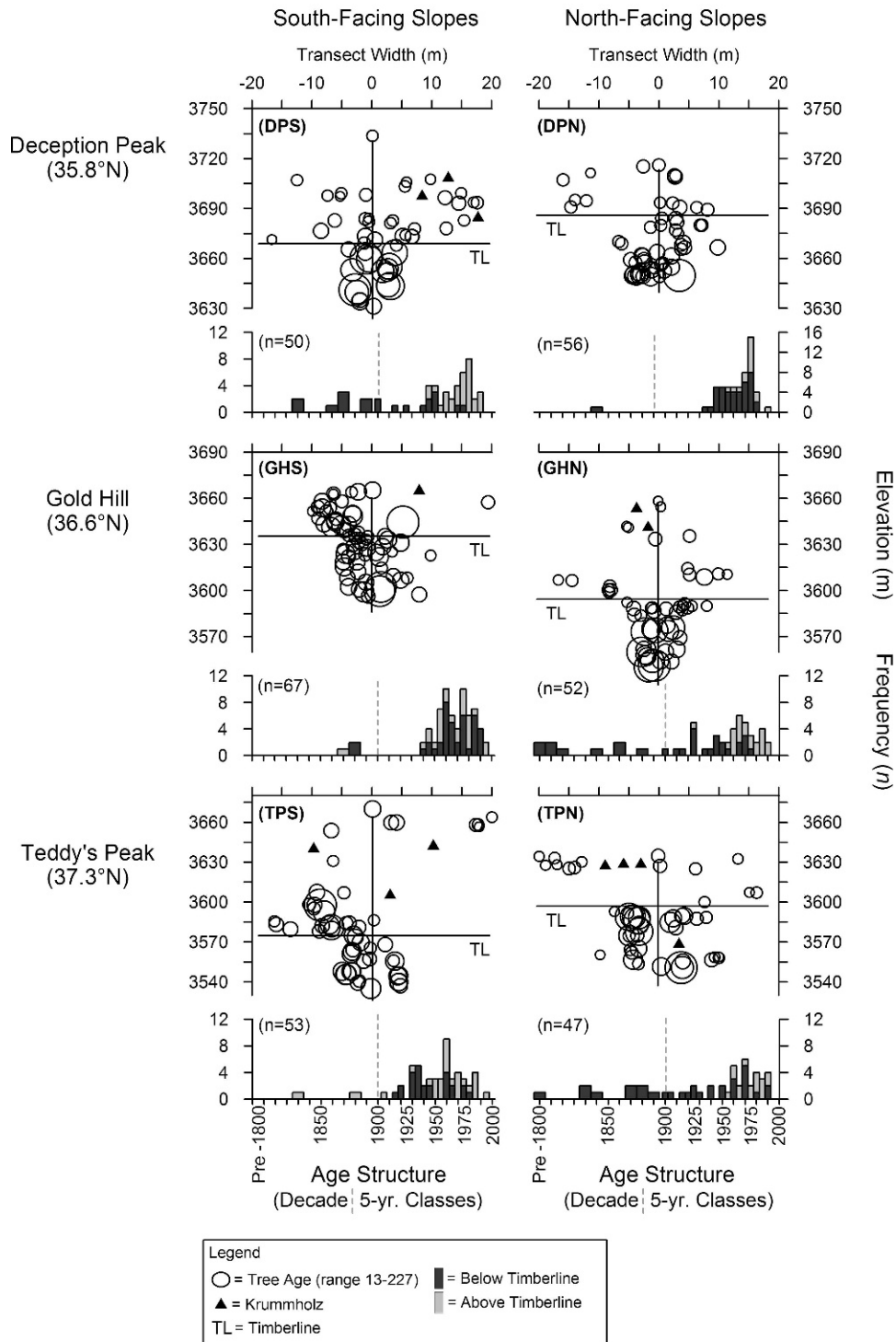
FIGURE 4. Spatial and temporal examination of upper treeline study sites in the Sangre de Cristo Mountains (SDC). Transects and age-structure data are shown for adjacent north- and south-facing slopes. The width of the nested-belt transect extended to 40 m above timberline and was reduced to 20 m below. The hybrid age-structure data is divided between decadal (pre-1800–1890) and 5-yr. (1900–2000) age classes. Note the different y-axis for age-structure of DPN. DP—Deception Peak; GH—Gold Hill; TP—Teddy's Peak.
