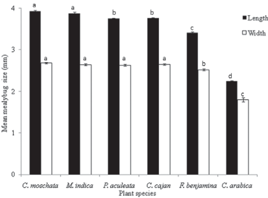
Fig. 2. Length and width (millimetres \pm SE) of adult female Rastrococcus iceryoides reared on 6 host plant species. For each parameter, bars sharing the letter do not differ significantly by Student–Newman–Keuls (SNK) test ( P = 0.05 ).
