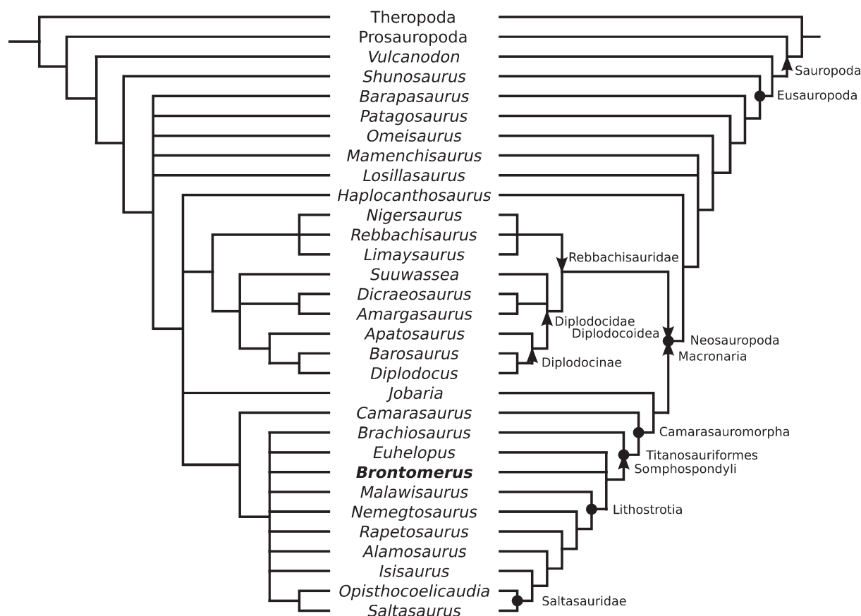
Fig. 11. Phylogenetic relationships of the camarasauromorph sauropod Brontomerus mcintoshi gen. et sp. nov. from the Lower Cretaceous Cedar Mountain Formation of Utah, produced using PAUP* 4.0b10 on the matrix of Harris (2006) augmented by Brontomerus , having 31 taxa and 331 characters. Left side, strict consensus of 180 most parsimonious trees (length = 788; CI = 0.5228; RI = 0.6848; RC = 0.3581); right side, 50% majority rule consensus.
