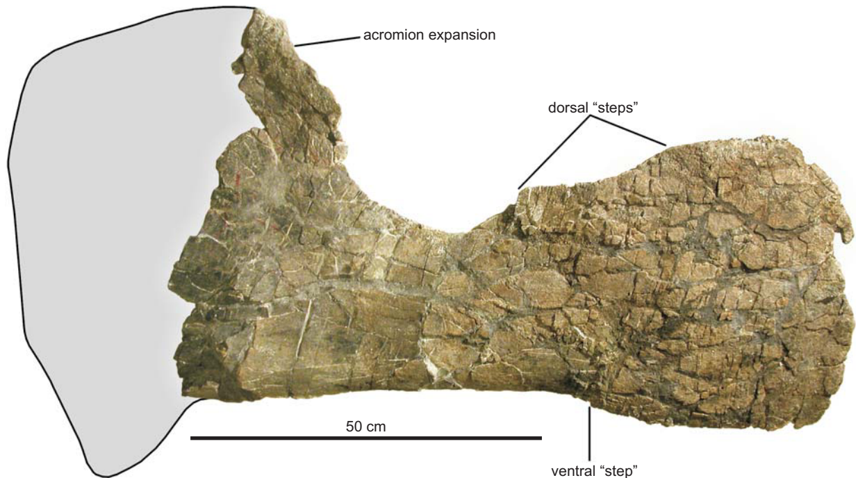
Fig. 8. Partial left scapula of the camarasauromorph sauropod Brontomerus mcintoshii gen. et sp. nov. from the Lower Cretaceous Cedar Mountain Formation of Utah, OMNH 27761, in lateral view, tentatively reconstructed after Giraffatitan brancai HMN Sa 9 (Janensch 1961: pl. 15: 1).
