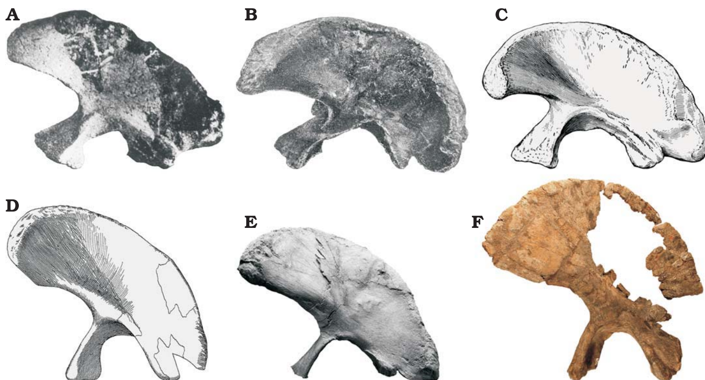
Fig. 3. Ili of sauropod dinosaurs, scaled to same total length. A. Mamenchisaurus hochuanensis Young and Zhao, 1972, holotype CCG V 20401, right ilium reversed, modified from Young and Zhao (1972: pl. 6: 1a). B. Diplodocus carnegii Hatcher, 1901, CM 94, right ilium reversed, modified from Hatcher (1901: pl. 10: 1). C. Camarasaurus supremus Cope, 1877, AMNH 5761 Il. 1, left ilium, modified from Osborn and Mook (1921: fig. 87). D. Giraffatitan brancai (Janensch, 1914), HMN J1, left ilium, modified from Janensch (1961: pl. E: 2). E. Rapetosaurus krausi Curry Rogers and Forster, 2001, holotype FMNH PR 2209, left ilium, modified from Curry Rogers (2009: fig. 39B). F. Brontomerus mcintoshii gen. et sp. nov. holotype OMNH 66430, left ilium.
