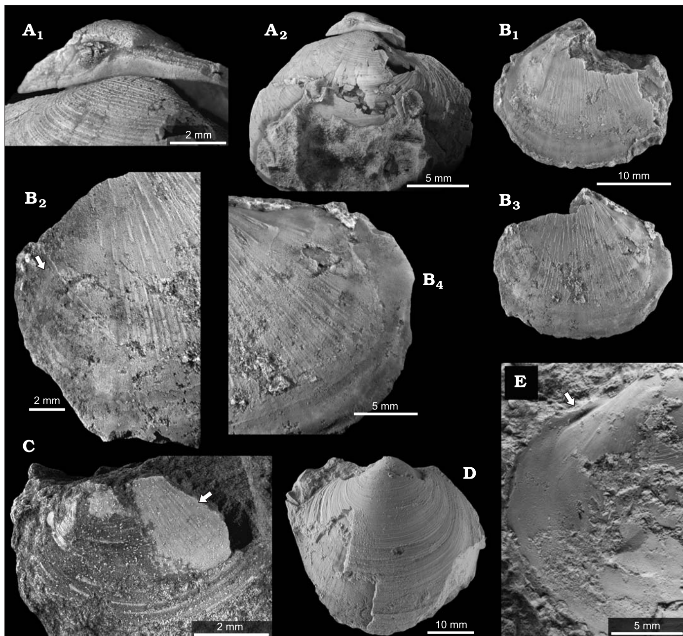
Fig. 7. Lucinidae from Cretaceous seep carbonates on Hokkaido, Japan. A, B. Nipponothracia yezoensis Kanie and Kuramochi, 1996 (Lucinidae) from the Cenomanian Kanajirisawa seep site on Hokkaido, Japan. A. Silicified specimen (UMUT MM 29541) showing the broad ligament ( A 1 ) and the edentulous hinge ( A 2 ). B. Internal mold (UMUT MM 29542) showing internal features, right and left valves ( B 1 , B 2 ), anterior part showing the elongate muscle scar ( B 3 , arrow), posterior part with muscle scar and pallial line ( B 4 ). C. Nipponothracia ponbetsensis Kanie and Sakai, 1997, from the Albian Ponbetsu site in Mikasa City; specimen (UMUT MM 29543) showing the radial internal ribs (arrow). D, E. Indetermined lucinid from the Cenomanian Kanajirisawa seep site. D. Large specimen (UMUT MM 29544) with nearly circular outline. E. Internal mold (UMUT MM 29545) showing faint radial sculpture, arrow indicates impression of lateral tooth.
