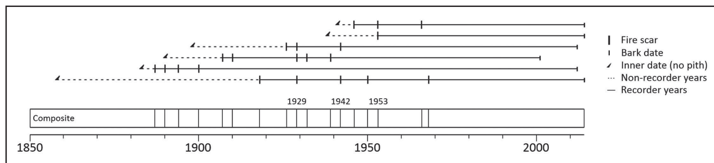
Figure 3. Fire history chart for the Glade Creek (GLDE) site at Babcock State Park, Fayette County, West Virginia. Each horizontal line represents a fire-scarred tree ( n = 6 ). The composite fire chronology highlights all years in which one tree recorded a fire, while years in which at least two trees recorded a fire are labeled.
