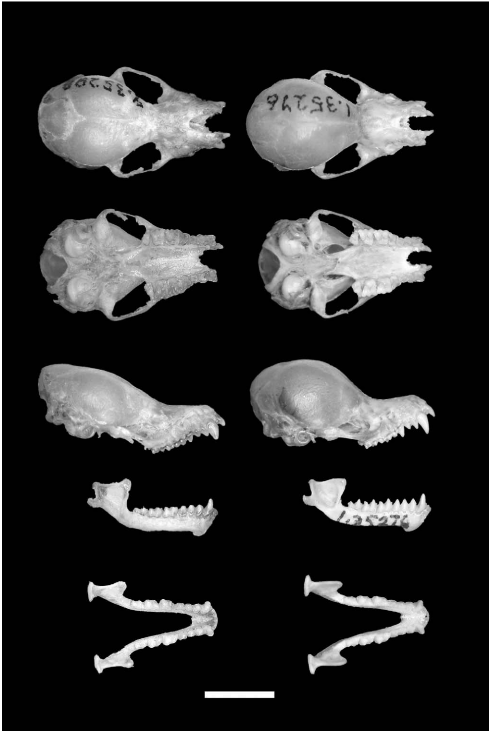
FIG. 1. Dorsal, ventral and lateral views of the cranium, and lateral and dorsal views of the mandible of (left) Kerivoula kachinensis , HBM.1.35288, Kachin, Myanmar and (right) K. lenis , HBM.1.35276, Tamil Nadu, India. Scale = 5 mm
