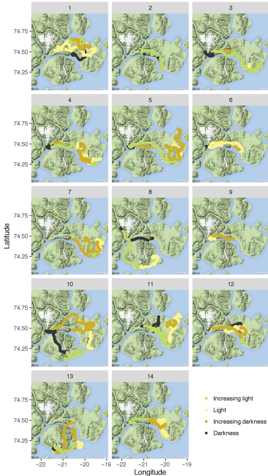
Figure 2. Overview of GPS locations for each of the 14 adult female muskoxen collared at Zackenberg in high-arctic Greenland during a full year. Numbers above panels refer to the identification numbers. Location data are broken down into four periods according to the light regime.
