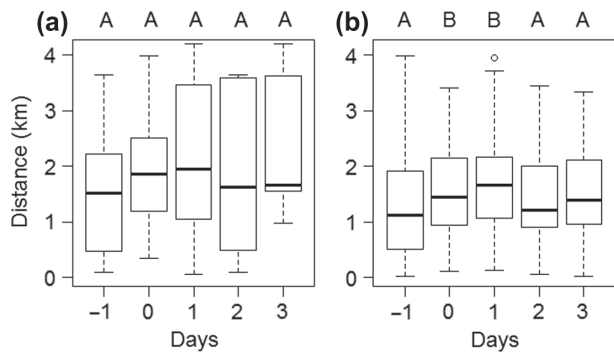
Figure 6. Effect of single hunting days on the local distribution of pink-footed goose flocks at Nesser in mid-Norway, 2011–2013, expressed by the distance (km) from hunting site to goose flocks the day before hunting (–1), on the day of hunting (0) and 1–3 days after hunting (1–3), for hunting days with a) few shots used (1–10) and b) many shots used (>10). Vertical lines represent minimum and maximum, boxes are interquartile ranges, horizontal lines medians and open dots outliers. Labels (A, B) show whether there is a significant difference (different letters) in median distance or not (same letters).
