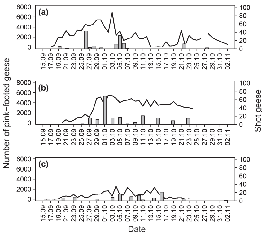
Figure 2. Number of pink-footed geese observed (black lines) and shot per day (grey columns) during 16 September to 3 November at Nesset in mid-Norway in (a) 2011, (b) 2012 and (c) 2013.
