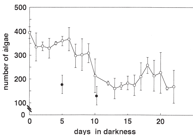
FIG. 1. Number of symbiotic algae per paramecium (2 stocks; OK-312 (●) and H-4 (○)) which were cultured under the condition of prolonged starvation in continuous darkness. Abscissa : days in continuous darkness; ordinate : mean number of symbiotic algae in green paramecium. Vertical bars denote one standard error. The average number of symbiotic algae per paramecium (in both 2 strains) gradually decreased until 10 days in darkness and thereafter kept constant. Results were expressed as the mean of 2 to 4 paramecia.
