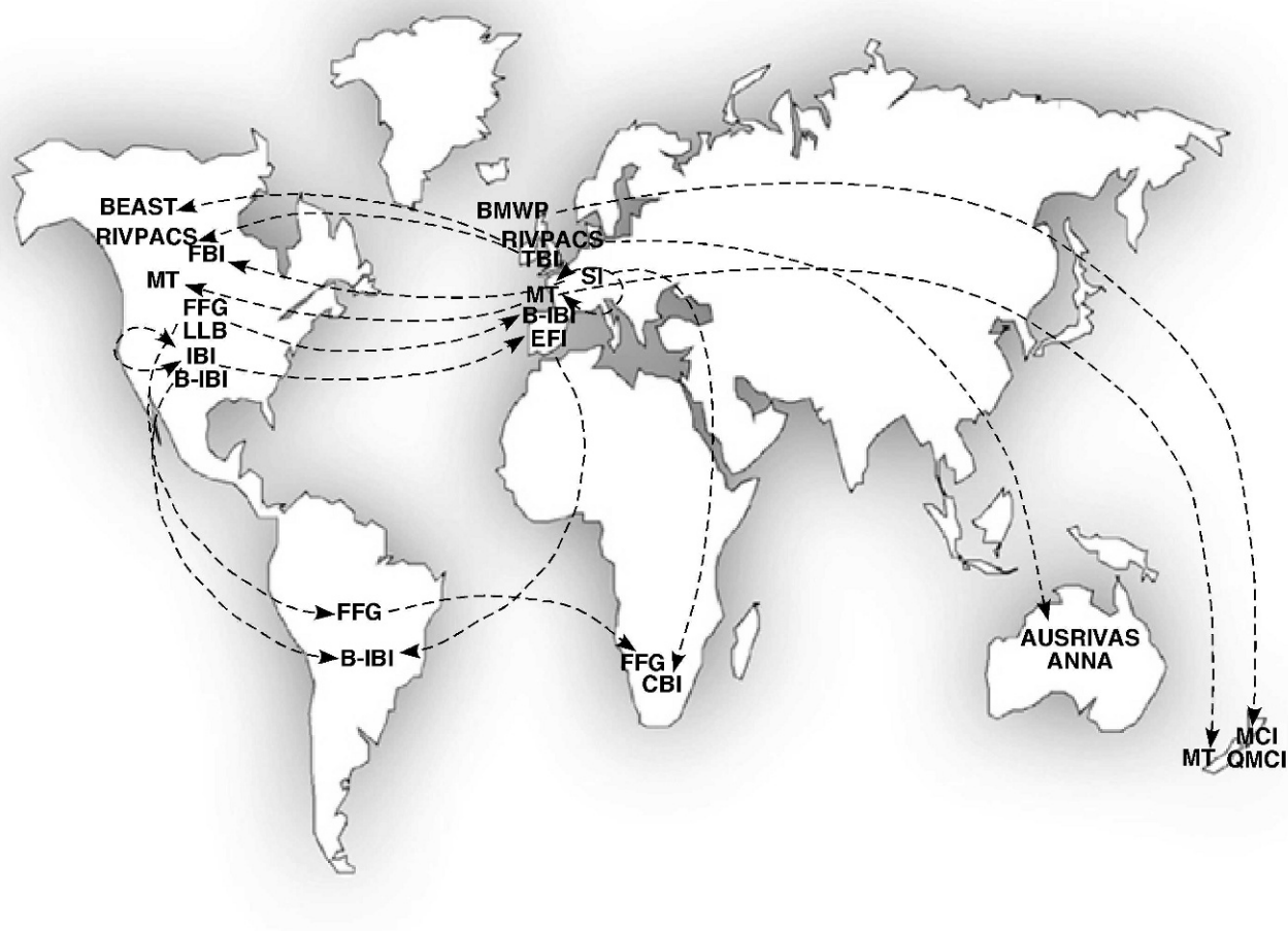
FIG. 2. Movements of selected bioassessment techniques from point of origin across the world. LLB = leaf litter breakdown, SP = secondary production, FFG = functional feeding group. See Appendix for abbreviations for bioassessment approaches.
