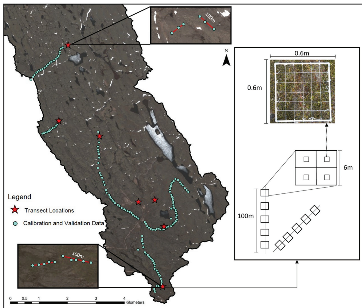
FIGURE 3. Sampling design for the Apex River Watershed (ARW). At seven sample sites, two 100-m transects were sampled using 6 m \times 6 m plots. At each plot, the center of each quadrant (3 m \times 3 m) was sampled with a 0.6 m \times 0.6 m quadrat to estimate percent vegetation cover (PVC). The number and orientation of transects varied at each location in order to sample across environmental and topographic gradients. Right inset—examples of the 0.6 m \times 0.6 m quadrats within each plot to determine PVC using the ITEX method. Additional calibration and validation data for image classification were collected while traveling from one transect location to another.
