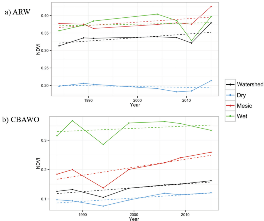
FIGURE 5. (a) NDVI time series by vegetation type in the ARW (1984–2015). The ARW represented in black contains all the usable pixels located in the watershed. (b) NDVI time series by vegetation type in the CBAWO (1985–2015). The CBAWO represented in black contains all the usable pixels located in the watershed.
