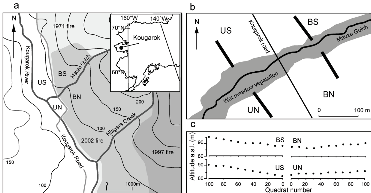
FIGURE 1. (a) Location of the study area. The four study sites are located in the Kougark area ( 65^{\circ}25'N , 164^{\circ}38'W ) in the center of the Seward Peninsula, Alaska. Kougark Road and Mauze Gulch form boundaries between the four experimental sites: BN (burned northwest-facing slope), BS (burned southeast-facing slope), UN (unburned northwest-facing slope), and US (unburned southeast-facing slope). The gray area shows the burned zones from the 1971, 1997, and 2002 fires. (b) A line transect was established at each of the four sites, and eleven 1 \times 1 m quadrats were set at a 10 m interval along each transect. (c) The profile of each site is shown along with each of the four transects.
