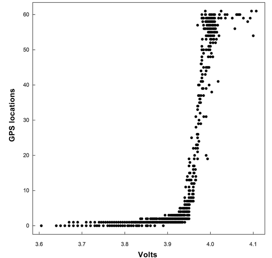
FIGURE 3. Hourly mean battery voltage and number of GPS locations collected for 3 GPS-GSM transmitters during 24 days of static testing on the ground in open fields, under forest cover, and suspended 11 m above the ground in an open field. Results are for all 3 transmitters combined.
