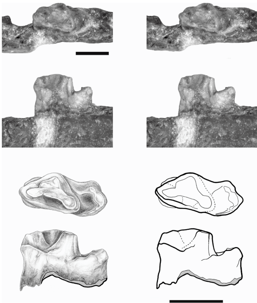
Fig. 7. Henosferus molus holotype MEFP 2353. Stereophotograph of the m1 in lingual and occlusal views, with accompanying drawings. Scale bar represents 1 mm.
