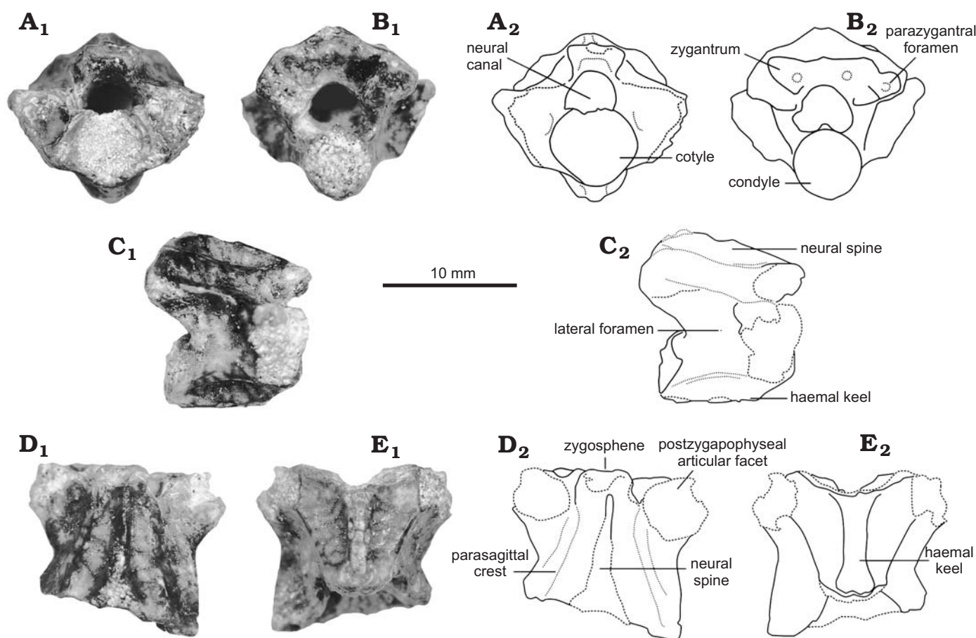
Fig. 3. Midtrunk vertebra of the snake cf. Seismophis septentrionalis sp. nov. (CPHNA-MA VT 1222), from the Cenomanian (early Late Cretaceous) of Falésia do Sismo, Cajual Island, Maranhão, northeastern Brazil. Photographs (A 1 –E 1 ) and explanatory drawings (A 2 –E 2 ), in anterior (A), posterior (B), lateral (C), dorsal (D), and ventral (E) views.
