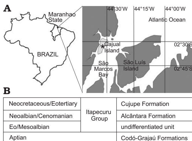
Fig. 1. A. Location map of Cajual Island. Asterisk shows Falésia do Sismo locality. B. Stratigraphy of São Luís-Grajaú Basin (modified from Rossetti 2001).
