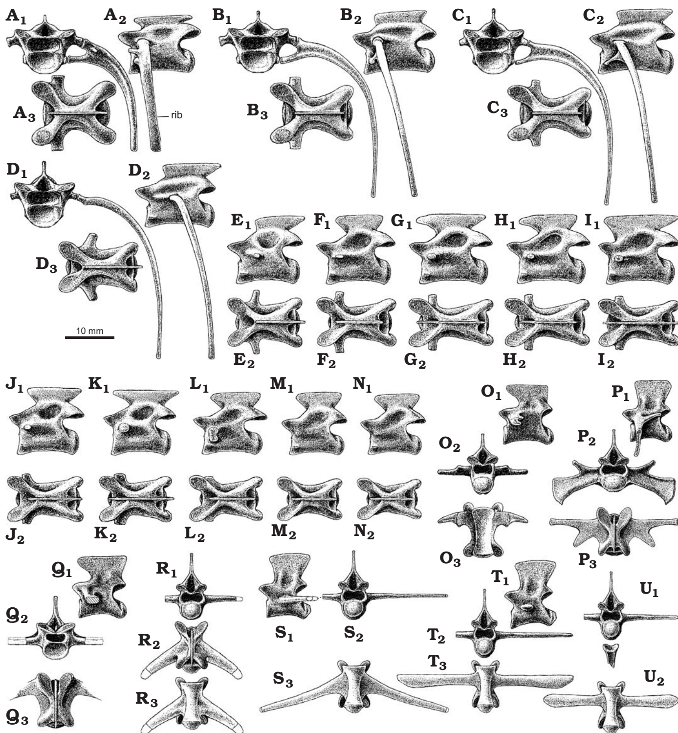
Fig. 10. Restoration of postcervical vertebrae of long-necked reptile Ozimek volans gen. et sp. nov. Dorsal 1 with ribs (A), dorsals 2–16 (B–N), based on ZPAL AbIII/2511, /2512, /3191. Sacrals 1–3 (O–Q), based on ZPAL AbIII/2511. Caudals 1, 2, 4 (R–T), caudal 6 with chevron (U), based on ZPAL AbIII/2512. In anterior (A 1 –D 1 , P 2 , Q 2 ), left lateral (A 2 –D 2 , E 1 –T 1 ), and dorsal (A 3 –D 3 , E 2 –N 2 , P 3 –R 3 ), posterior (O 2 , P 2 , R 2 , S 2 , T 2 , U 1 ), and ventral (O 3 , R 4 , S 3 , T 3 , U 2 ) views.
