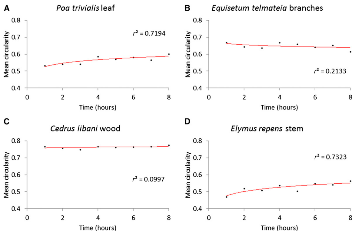
Fig. 5. Relationships between mean circularity and duration of simulated transport for charcoal particles ( 315\text{--}1,000,000\text{ }\mu\text{m}^2 ) produced from four of the plant materials. Logarithmic models and associated coefficients of determination ( r^2 ) are also shown. Poa trivialis (A) is typical of the leaves (median r^2 ), showing an increase in mean circularity with increasing transport time. Although all true leaves displayed this tendency, charcoal particles from branches of Equisetum telmateia (B) did not. Stem samples showed no overall trends, with low coefficients of determination and inconsistent direction of change, with Cedrus libani (C) being typical (closest to median r^2 ). Elymus repens (D) was one of only two specimens that did have a reasonable model fit, showing increasing circularity with transport time.
