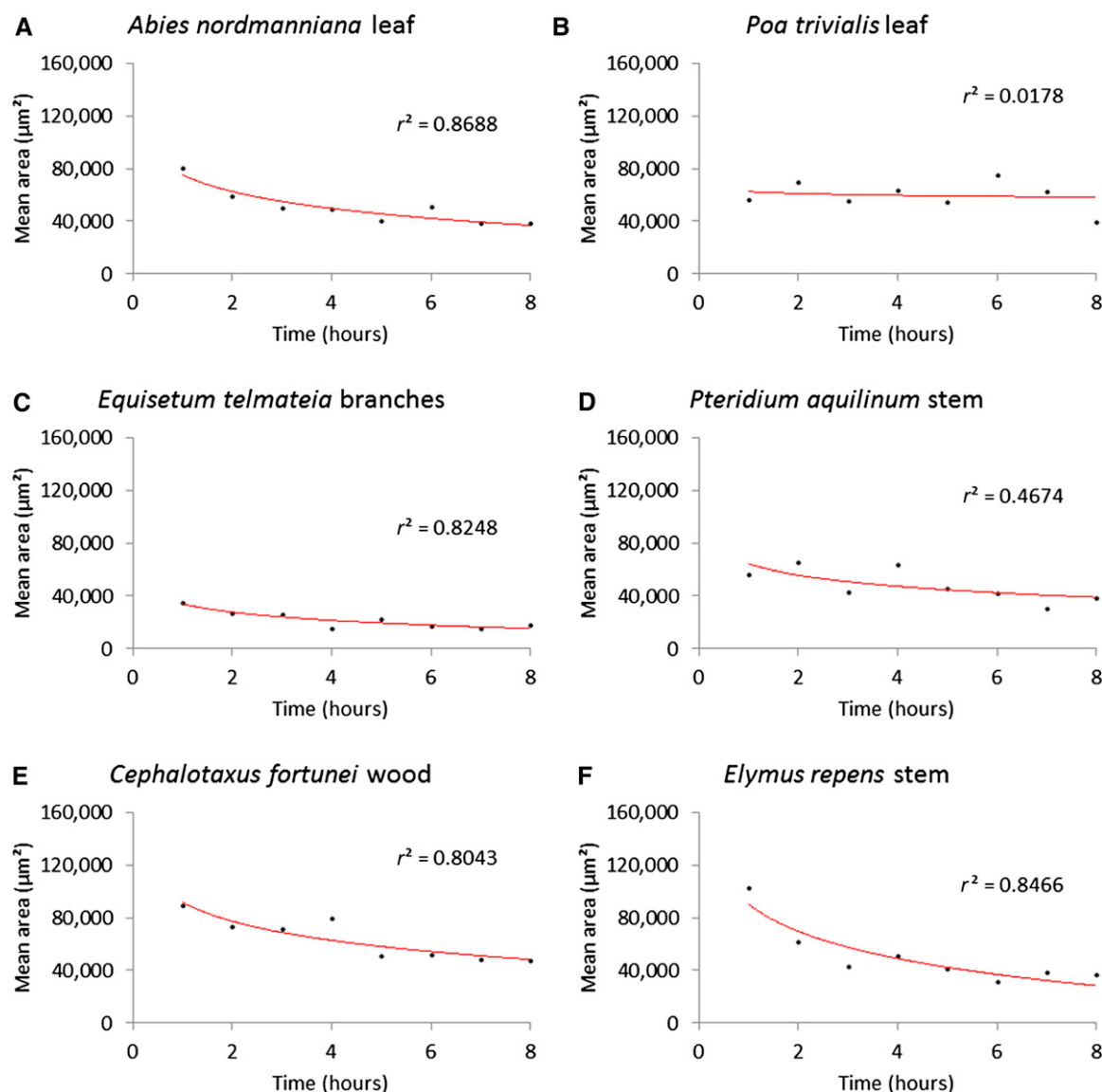
Fig. 4. Relationships between mean projected area and duration of simulated transport for charcoal particles ( 315\text{--}1,000,000\ \mu\text{m}^2 ) produced from six of the plant materials. Logarithmic models and associated coefficients of determination ( r^2 ) are also shown. Abies nordmanniana (A) is typical of the leaves (median r^2 ), showing mean particle area as a logarithmic function of transportation time; Poa trivialis (B) was the only leaf that did not display such a trend, although branches of Equisetum telmateia (C) did display this trend. Pteridium aquilinum (D) is typical of the stem samples (closest to median r^2 ) in fitting the logarithmic model poorly; Cephalotaxus fortunei (E) and Elymus repens (F) were exceptions to this.
