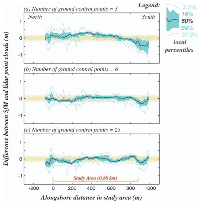
Figure 8. Summary of the alongshore differences between the SfM-derived point clouds and airborne LIDAR along the Fort Funston study area during 2010 for the same examples shown in Figure 7. Data are presented as percentiles of all difference measurements within 10-m alongshore increments. Measurements on the trees and beach were removed to eliminate the bias these observations added. Results shown for (a) 3, (b) 6, and (c) 25 ground control points. The area of \pm 0.2 m is highlighted with solid yellow. (Color for this figure is available in the online version of this paper.)
