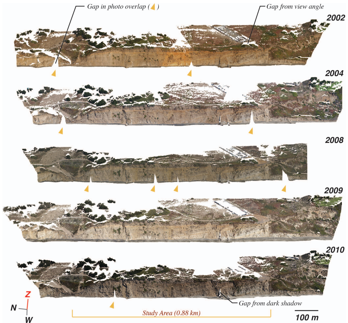
Figure 4. Three-dimensional point clouds generated for the Fort Funston study area using SfM and 5 years of oblique historical photos. Gaps in the point clouds were caused by either gaps in photo overlaps (yellow arrows), ground areas unseen in the imagery owing to view angle, or areas masked by dark shadows.
