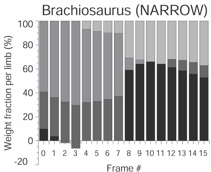
FIGURE 8. Graphical views of the percentage of body weight carried by each Brachiosaurus limb at each stage of the narrow- and wide-gauge walk cycles illustrated in Figure 6. Each column of these plots contains the relative fractions of body weight born by all four limbs, and the combined result of all four limbs at each stage sums to 100% of the body weight. Summaries of the loadings are summarized in Table 3. The upper graph shows that when making the wide-gauge trackway all the loads on the limbs are positive and the model will not tip. The lower graph highlights the occurrence of periods of negative loading (Frame 3) during the attempt at producing a narrow-gauge trackway, which indicates that the model was unstable and starting to tip. As predicted by its more anteriorly placed CM, Brachiosaurus carries a greater fraction of its weight on its forelimbs than does Diplodocus (Fig. 9).
