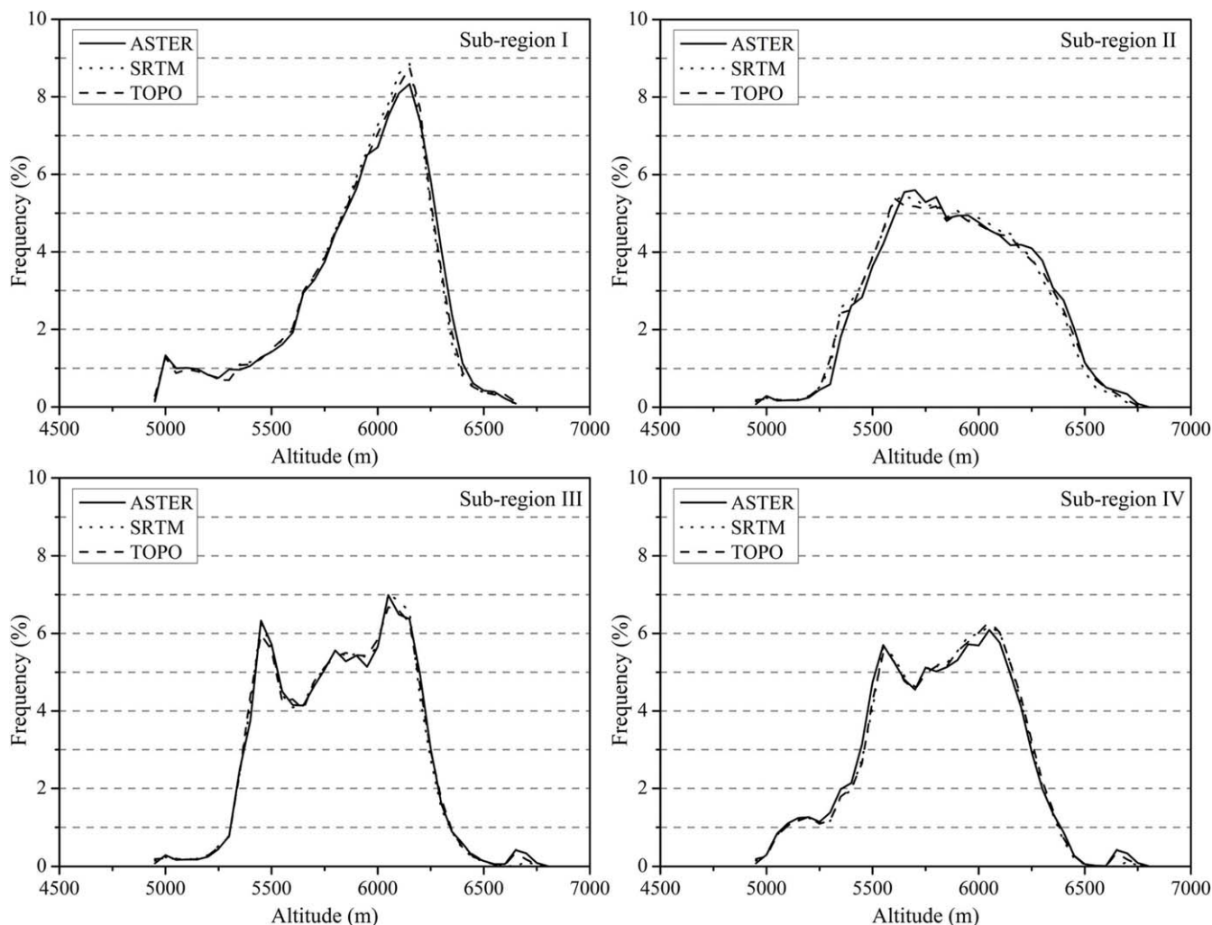
FIGURE 2. Histograms of elevation distributions for the multi-DEMs covering four subregions. The altitude interval is 50 m.
