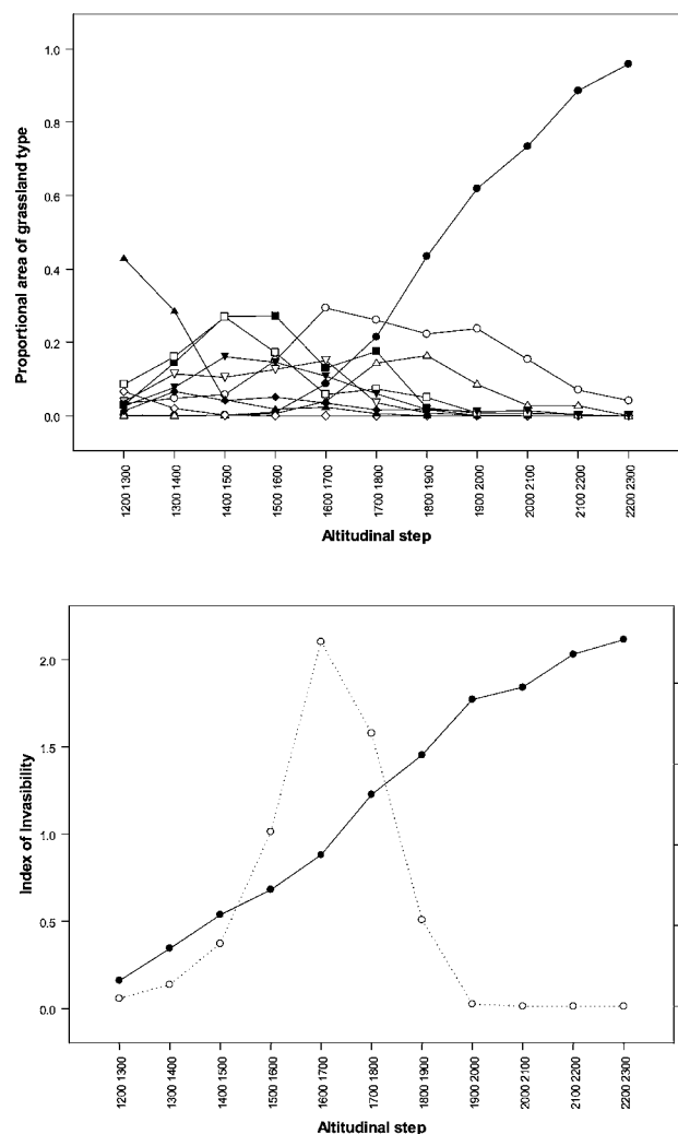
FIGURE 4. (top) Proportional area of the 10 predominant grassland communities of the study area in altitudinal steps of 100 m. \bullet = Carex firma grassland; \circ = Carex sempervirens grassland; \blacklozenge = Carex ferruginea grassland; \diamond = Calamagrostis varia grassland; \blacktriangle = Tall herb communities; \triangle = Agrostis alpina – Festuca pumila grassland; \blacktriangledown = Deschampsia cespitosa pasture; \nabla = Helictotrichon parlatorei grassland; \blacksquare = Leontodon hispidus – Crepis aurea pasture; \square = Nardus stricta pasture. (bottom) Index of invasibility of the overall grassland matrix (= sum of the proportional areas of the 10 predominant grassland types weighted by their respective index of invasibility (= solid line) and current distribution of Pinus mugo shrublands (= dotted line) in altitudinal steps of 100 m.
