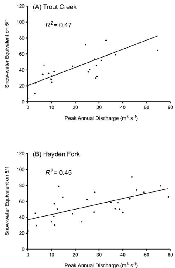
FIGURE 4. Relations between snow-water equivalent on May 1 and peak annual discharge for two representative pairs of SNOTEL stations and stream gages. (A) Trout Creek SNOTEL station and Ashley Creek gage station, and (B) Hayden Fork SNOTEL station and Bear River gage station.
