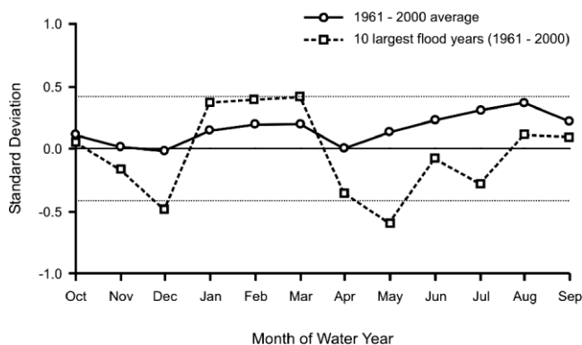
FIGURE 9. Monthly temperature anomalies in NCDC Utah climate division 5 for 1961–2000 and for the 10 largest flood years in 1961–2000, expressed in standard deviation departures from mean. Note that with the standardized series, the long-term (1900–2000) average for temperature is 0.0.
