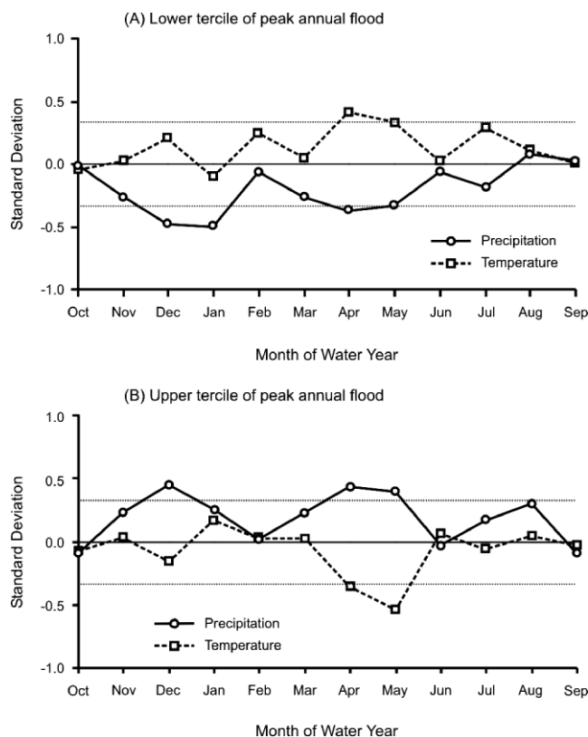
FIGURE 6. Composite precipitation and temperature standard deviation departures from mean in the Uinta Mountains for (A) low flood years and (B) high flood years. Climate data represents NCDC's Utah climate division 5 (mountainous northeastern Utah) for the period 1918–2000.
