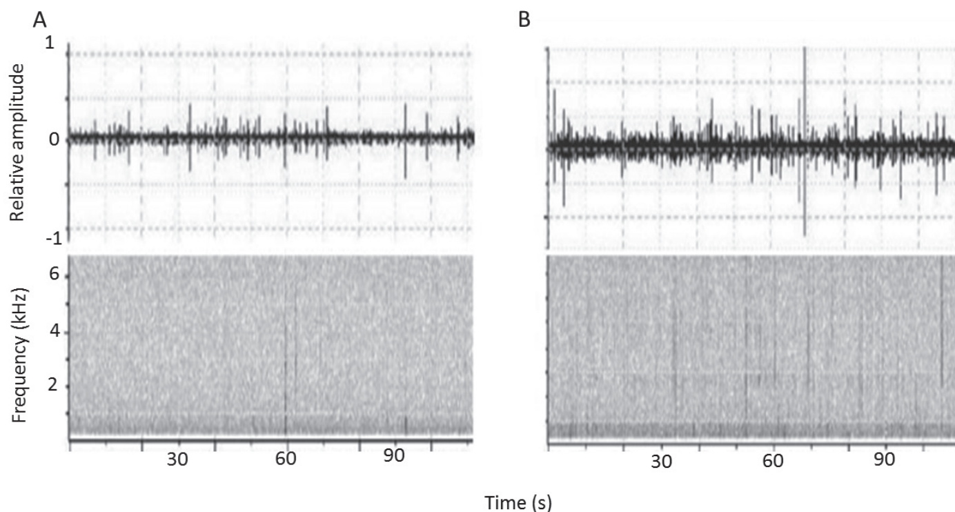
Fig. 2. Oscillograms and spectrograms of signals recorded from beans infested with A) adults and B) larvae of Acanthoscelides obtectus . Darker shade in spectrogram indicates greater energy at specified frequency and time.
