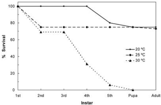
Fig. 1. Survival of Metriona elatior immatures at different temperatures.
