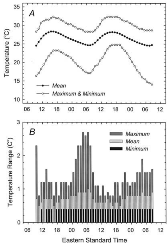
Fig. 6. Variation in temperature on the floor of the shed with time of day. (A) Mean, minimum, and maximum temperatures for each hour based on temperature records for all trap sites, replicates, and experiments combined (210 records). The maxima and minima for each time of day are the highest and lowest temperatures recorded for that time over the course of the entire study. (B) Mean, minimum, and maximum temperature ranges (differences between trap sites with the highest and lowest readings) for each time of day. Ranges were determined for each hour of each replicate, and all replicates were then combined to determine mean, minimum, and maximum ranges for the study. The range of each temperature statistic can be read from the top of the shading representing that statistic.
